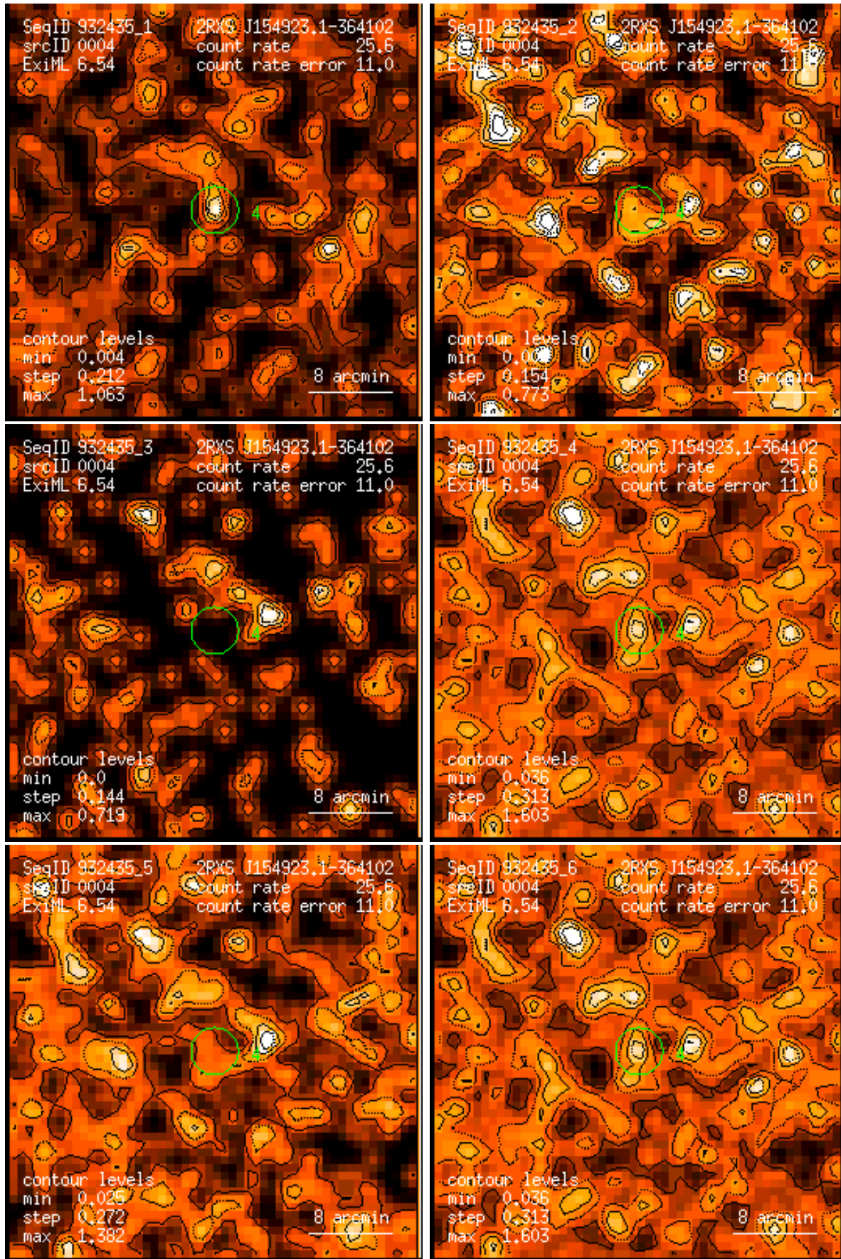
Figure 4: RASS 932435: detection 0004: band rate images, Gaussian filter: (1) PSPC channels 11 – 41, (2) 52 – 90, (3) 91 – 201, (4) 11 – 235, (5) 52 – 201, (6) 11 – 201. Broad band rates in counts/ks. Band rate contour levels in counts/ks/arcmin 2 .
