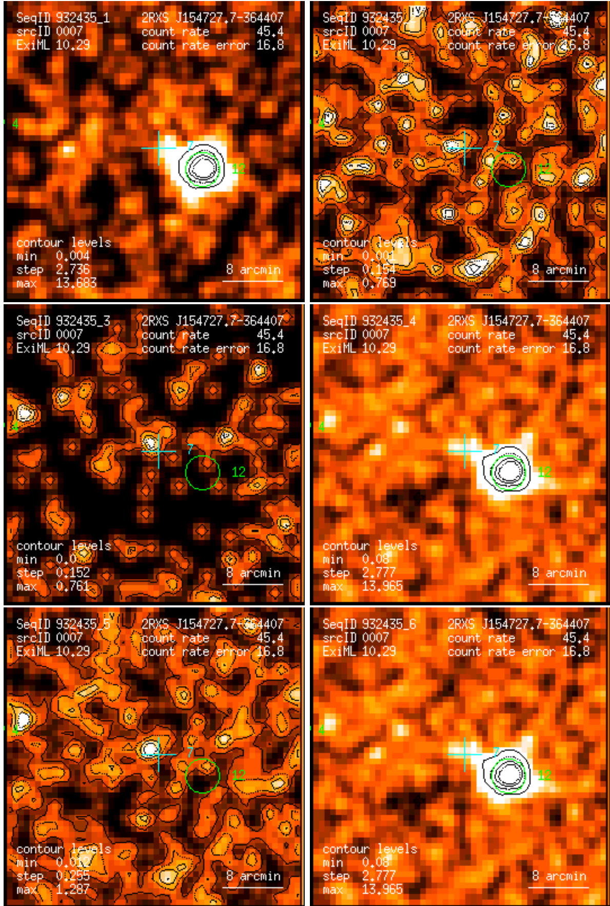
Figure 7: RASS 932435: detection 0007: band rate images, Gaussian filter: (1) PSPC channels 11 – 41, (2) 52 – 90, (3) 91 – 201, (4) 11 – 235, (5) 52 – 201, (6) 11 – 201. Broad band rates in counts/ks. Band rate contour levels in counts/ks/arcmin 2 .
