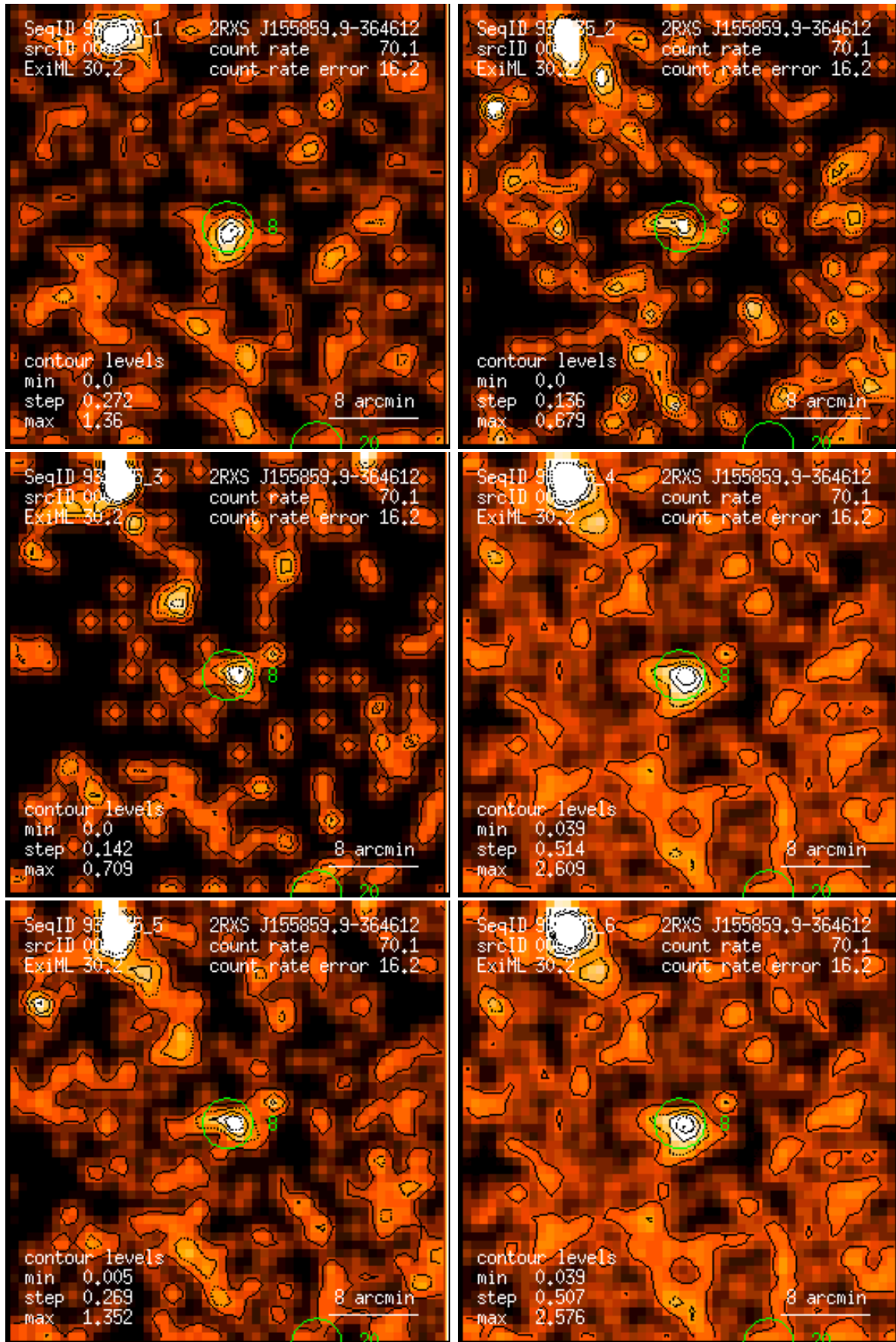
Figure 8: RASS 932435: detection 0008: band rate images, Gaussian filter: (1) PSPC channels 11 – 41, (2) 52 – 90, (3) 91 – 201, (4) 11 – 235, (5) 52 – 201, (6) 11 – 201. Broad band rates in counts/ks. Band rate contour levels in counts/ks/arcmin 2 .
