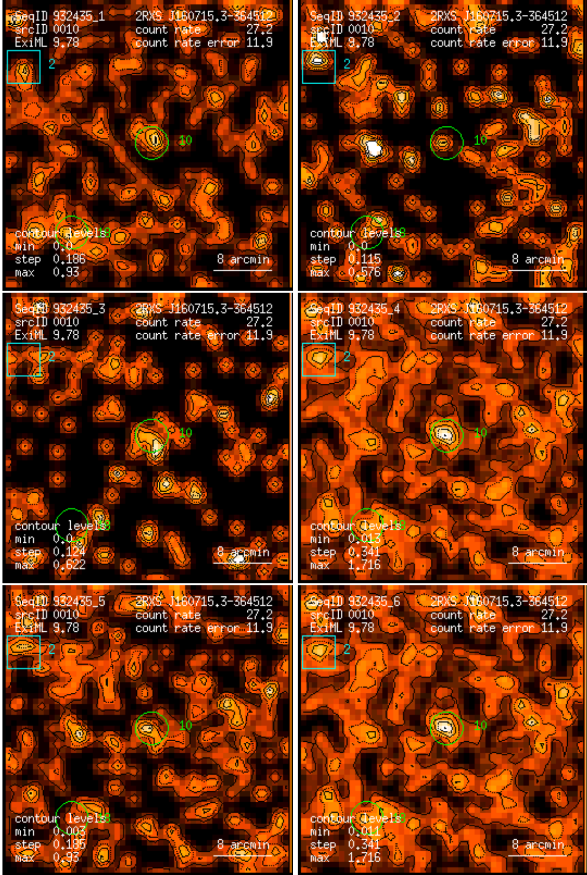
Figure 10: RASS 932435: detection 0010: band rate images, Gaussian filter: (1) PSPC channels 11 – 41, (2) 52 – 90, (3) 91 – 201, (4) 11 – 235, (5) 52 – 201, (6) 11 – 201. Broad band rates in counts/ks. Band rate contour levels in counts/ks/arcmin 2 .
