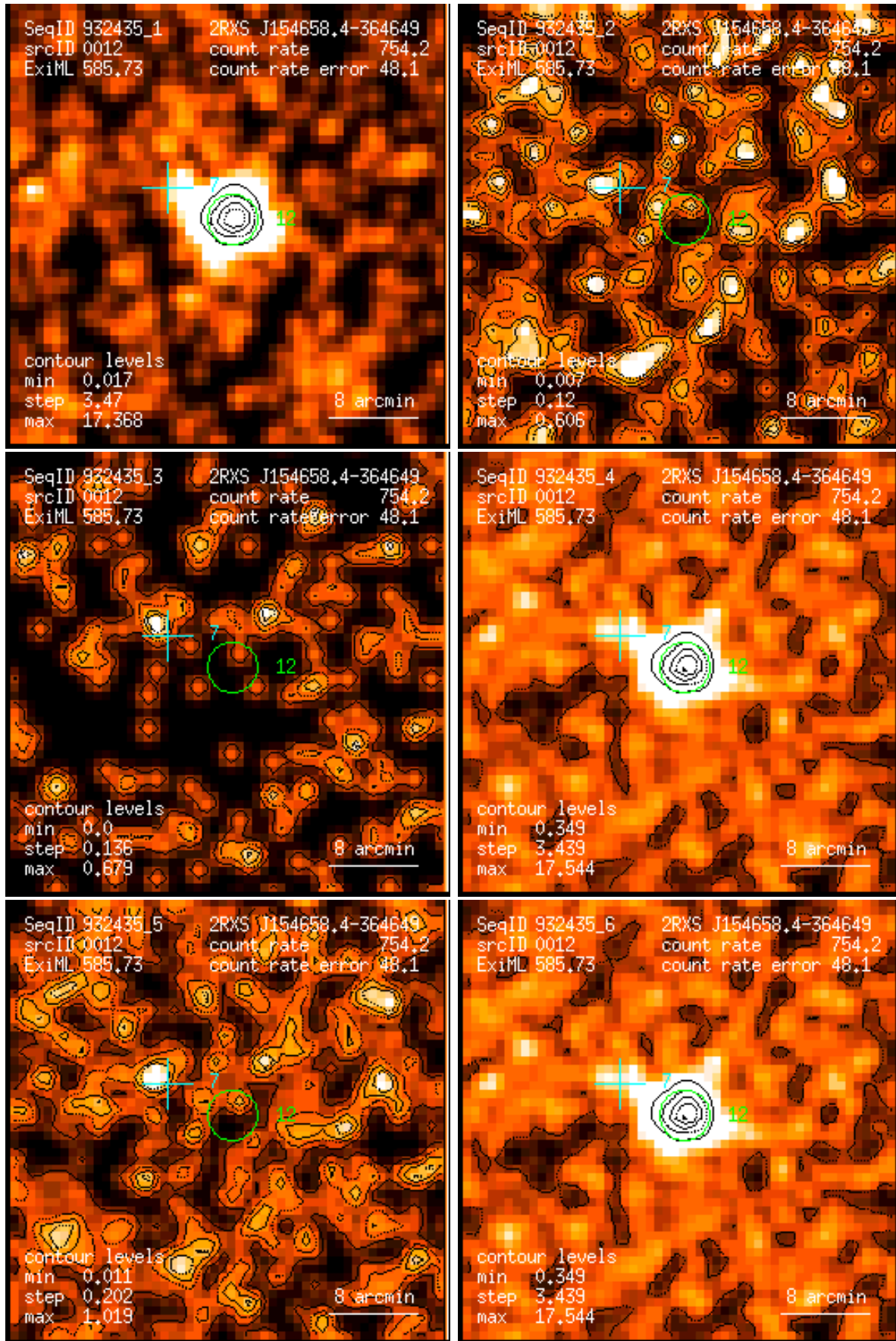
Figure 12: RASS 932435: detection 0012: band rate images, Gaussian filter: (1) PSPC channels 11 – 41, (2) 52 – 90, (3) 91 – 201, (4) 11 – 235, (5) 52 – 201, (6) 11 – 201. Broad band rates in counts/ks. Band rate contour levels in counts/ks/arcmin 2 .
