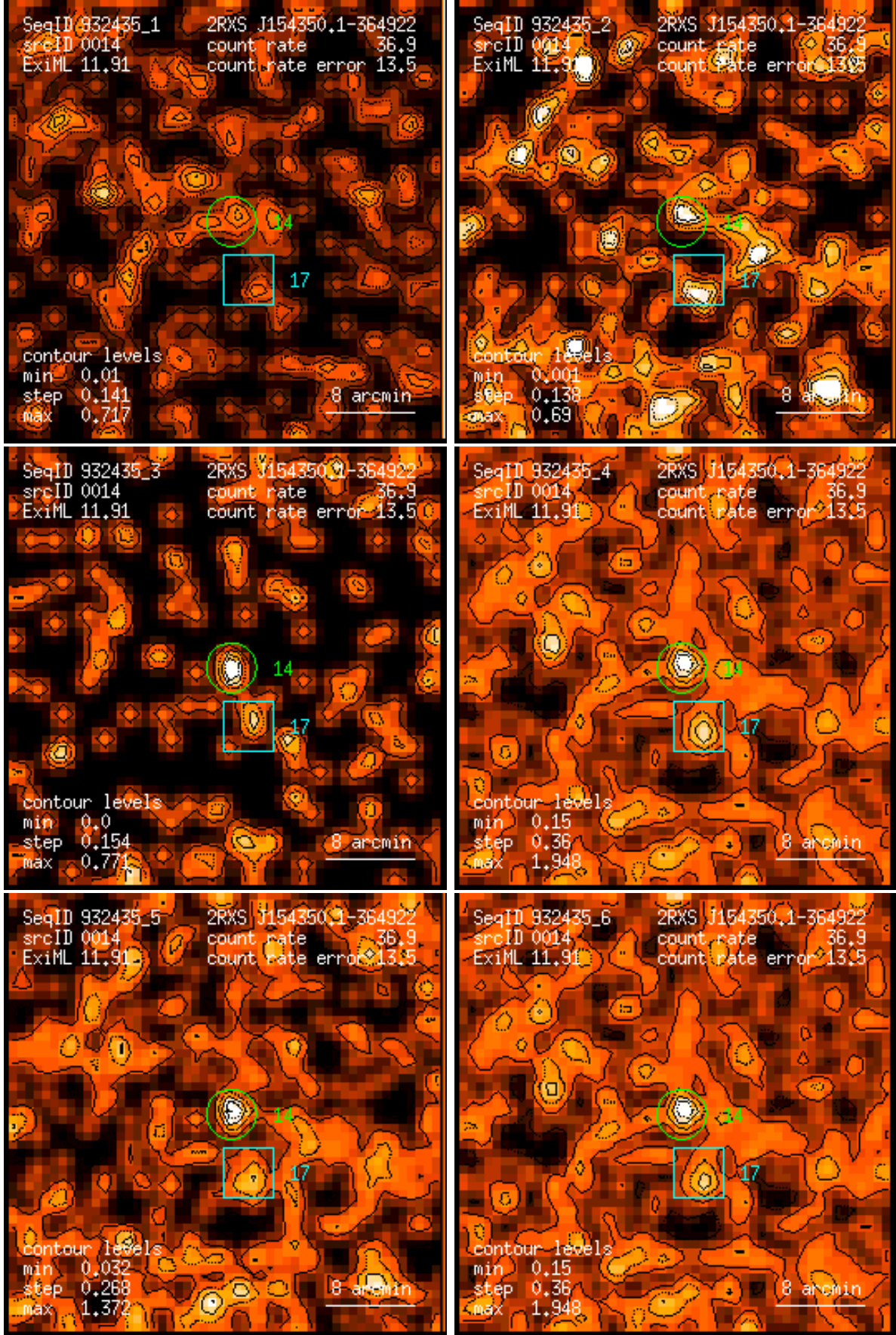
Figure 14: RASS 932435: detection 0014: band rate images, Gaussian filter: (1) PSPC channels 11 – 41, (2) 52 – 90, (3) 91 – 201, (4) 11 – 235, (5) 52 – 201, (6) 11 – 201. Broad band rates in counts/ks. Band rate contour levels in counts/ks/arcmin 2 .
