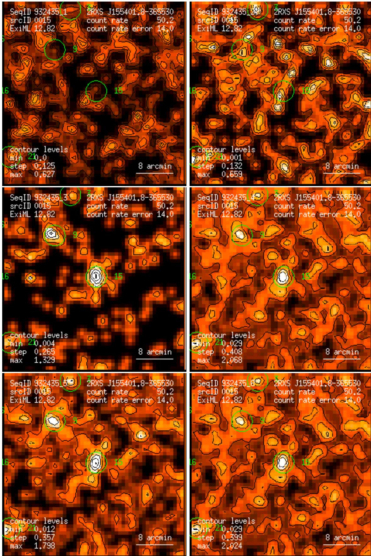
Figure 15: RASS 932435: detection 0015: band rate images, Gaussian filter: (1) PSPC channels 11 – 41, (2) 52 – 90, (3) 91 – 201, (4) 11 – 235, (5) 52 – 201, (6) 11 – 201. Broad band rates in counts/ks. Band rate contour levels in counts/ks/arcmin 2 .
