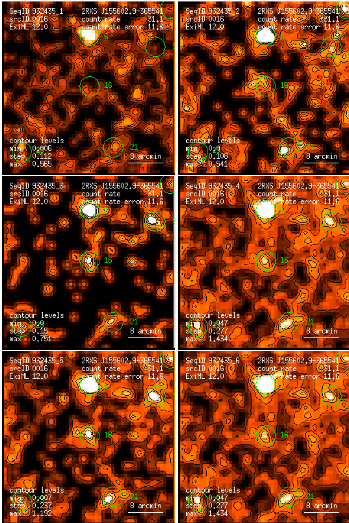
Figure 16: RASS 932435: detection 0016: band rate images, Gaussian filter: (1) PSPC channels 11 – 41, (2) 52 – 90, (3) 91 – 201, (4) 11 – 235, (5) 52 – 201, (6) 11 – 201. Broad band rates in counts/ks. Band rate contour levels in counts/ks/arcmin 2 .
