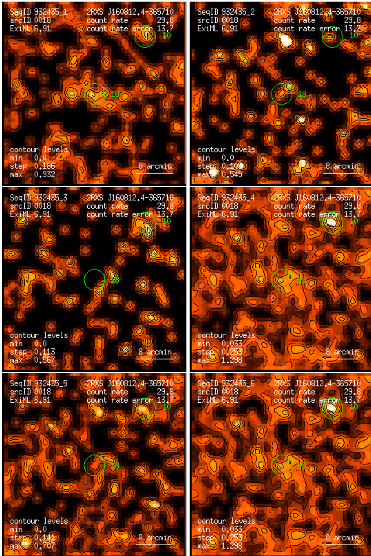
Figure 18: RASS 932435: detection 0018: band rate images, Gaussian filter: (1) PSPC channels 11 – 41, (2) 52 – 90, (3) 91 – 201, (4) 11 – 235, (5) 52 – 201, (6) 11 – 201. Broad band rates in counts/ks. Band rate contour levels in counts/ks/arcmin 2 .
