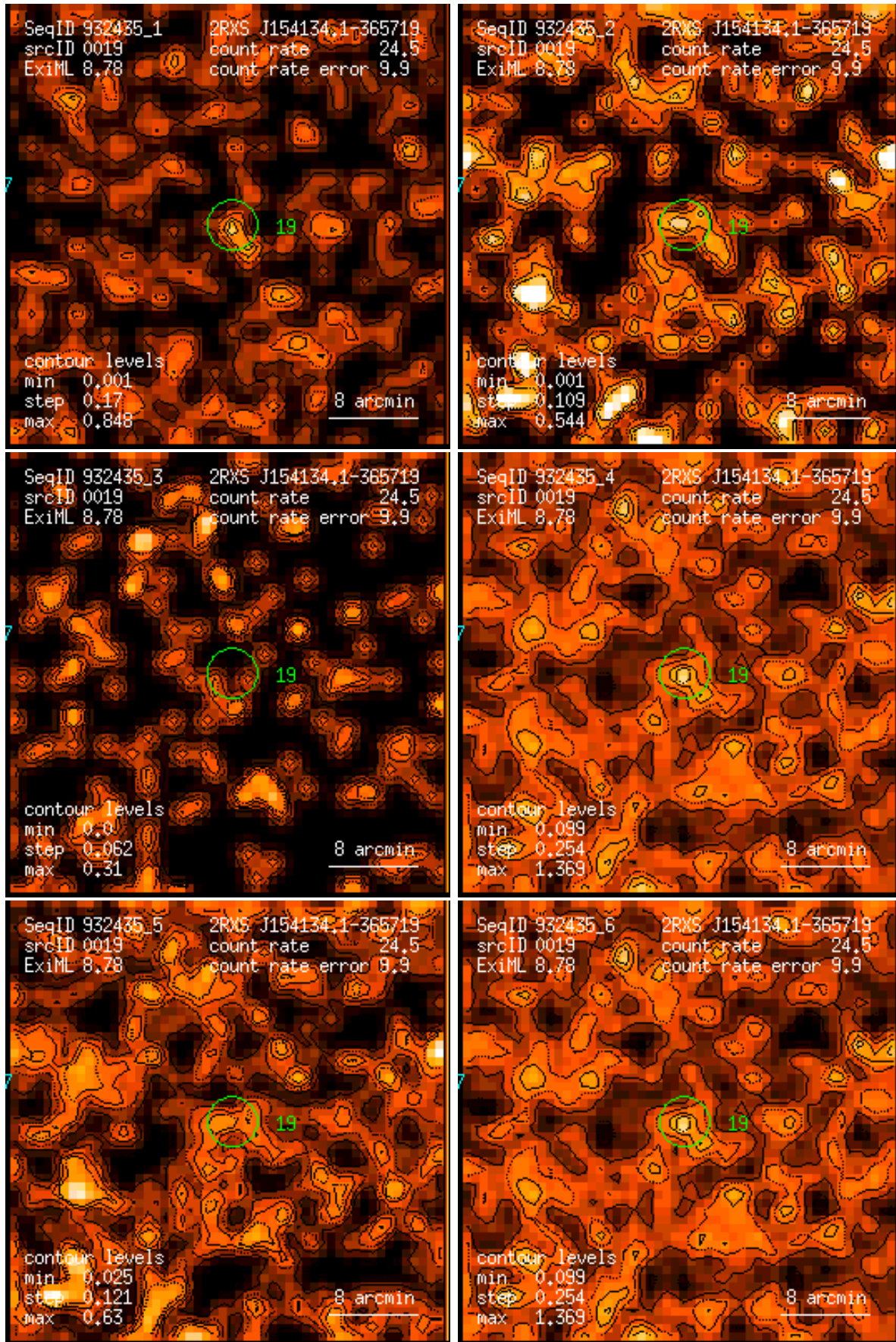
Figure 19: RASS 932435: detection 0019: band rate images, Gaussian filter: (1) PSPC channels 11 – 41, (2) 52 – 90, (3) 91 – 201, (4) 11 – 235, (5) 52 – 201, (6) 11 – 201. Broad band rates in counts/ks. Band rate contour levels in counts/ks/arcmin 2 .
