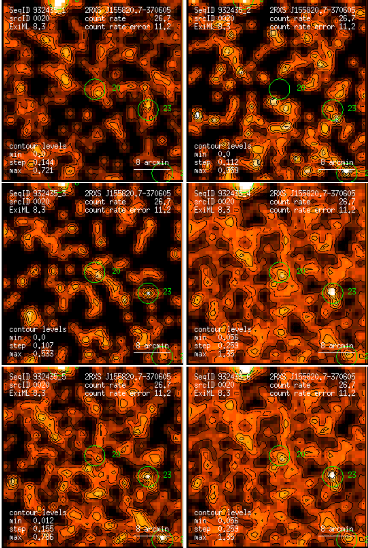
Figure 20: RASS 932435: detection 0020: band rate images, Gaussian filter: (1) PSPC channels 11 – 41, (2) 52 – 90, (3) 91 – 201, (4) 11 – 235, (5) 52 – 201, (6) 11 – 201. Broad band rates in counts/ks. Band rate contour levels in counts/ks/arcmin 2 .
