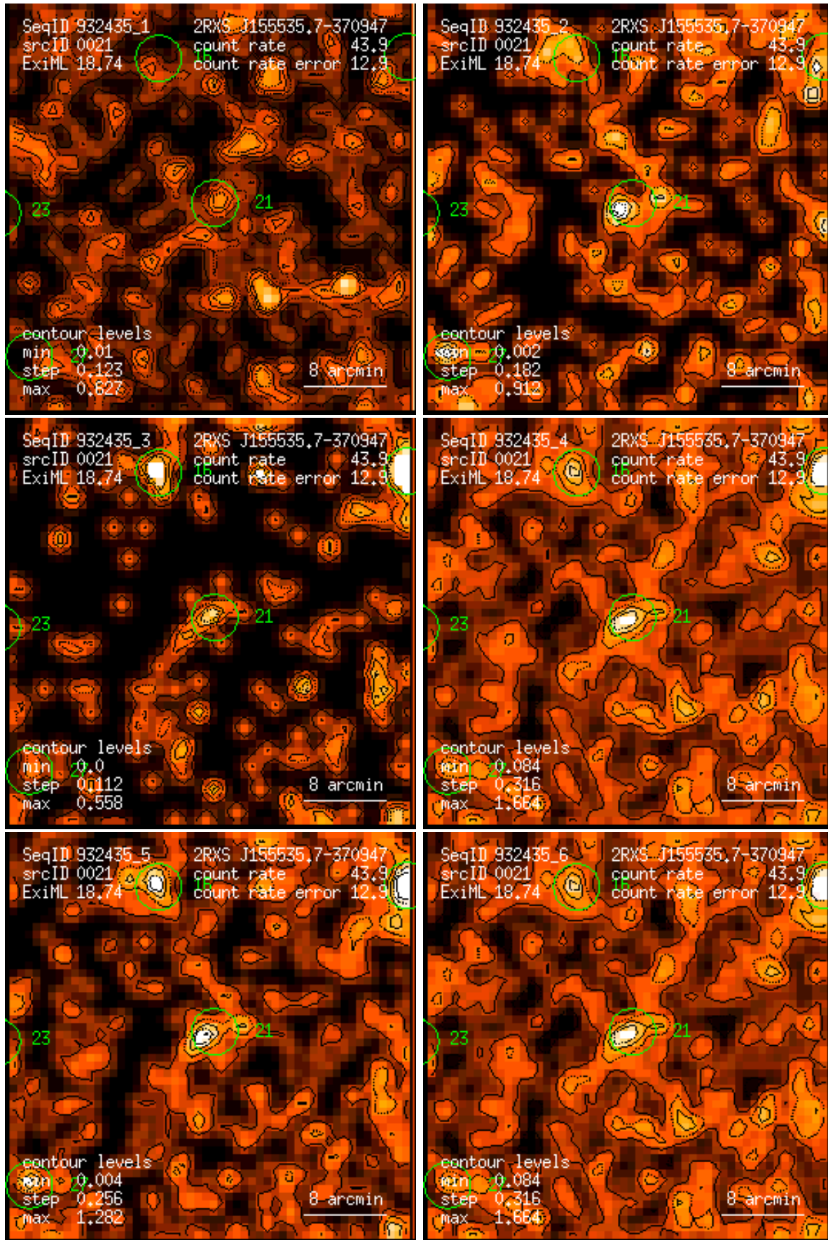
Figure 21: RASS 932435: detection 0021: band rate images, Gaussian filter: (1) PSPC channels 11 – 41, (2) 52 – 90, (3) 91 – 201, (4) 11 – 235, (5) 52 – 201, (6) 11 – 201. Broad band rates in counts/ks. Band rate contour levels in counts/ks/arcmin 2 .
