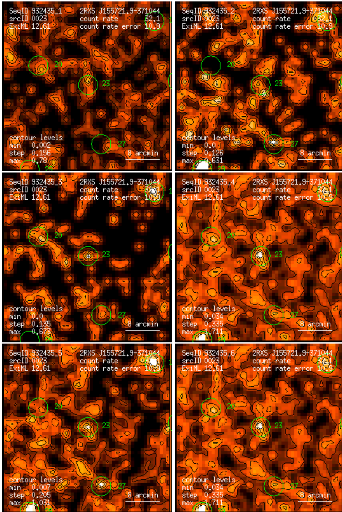
Figure 23: RASS 932435: detection 0023: band rate images, Gaussian filter: (1) PSPC channels 11 – 41, (2) 52 – 90, (3) 91 – 201, (4) 11 – 235, (5) 52 – 201, (6) 11 – 201. Broad band rates in counts/ks. Band rate contour levels in counts/ks/arcmin 2 .
