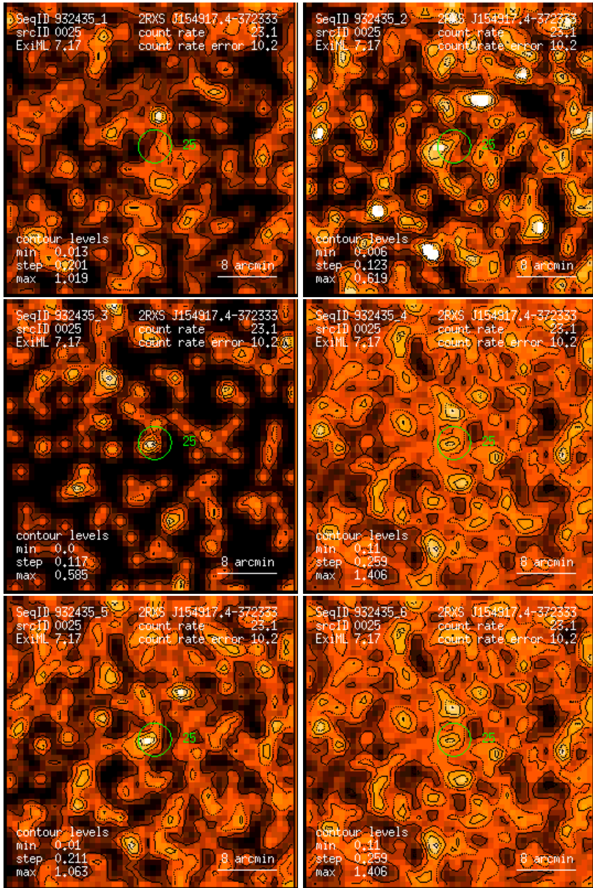
Figure 25: RASS 932435: detection 0025: band rate images, Gaussian filter: (1) PSPC channels 11 – 41, (2) 52 – 90, (3) 91 – 201, (4) 11 – 235, (5) 52 – 201, (6) 11 – 201. Broad band rates in counts/ks. Band rate contour levels in counts/ks/arcmin 2 .
