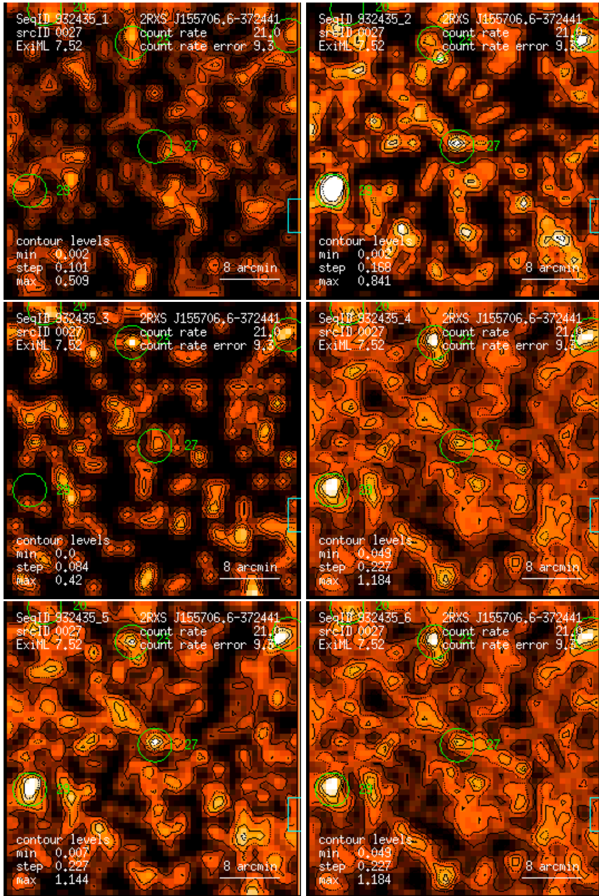
Figure 27: RASS 932435: detection 0027: band rate images, Gaussian filter: (1) PSPC channels 11 – 41, (2) 52 – 90, (3) 91 – 201, (4) 11 – 235, (5) 52 – 201, (6) 11 – 201. Broad band rates in counts/ks. Band rate contour levels in counts/ks/arcmin 2 .
