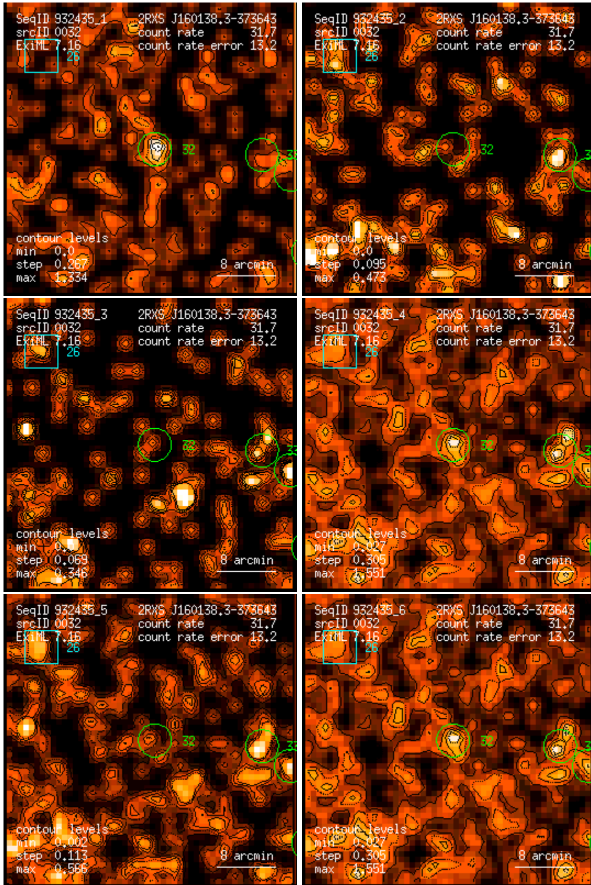
Figure 32: RASS 932435: detection 0032: band rate images, Gaussian filter: (1) PSPC channels 11 – 41, (2) 52 – 90, (3) 91 – 201, (4) 11 – 235, (5) 52 – 201, (6) 11 – 201. Broad band rates in counts/ks. Band rate contour levels in counts/ks/arcmin 2 .
