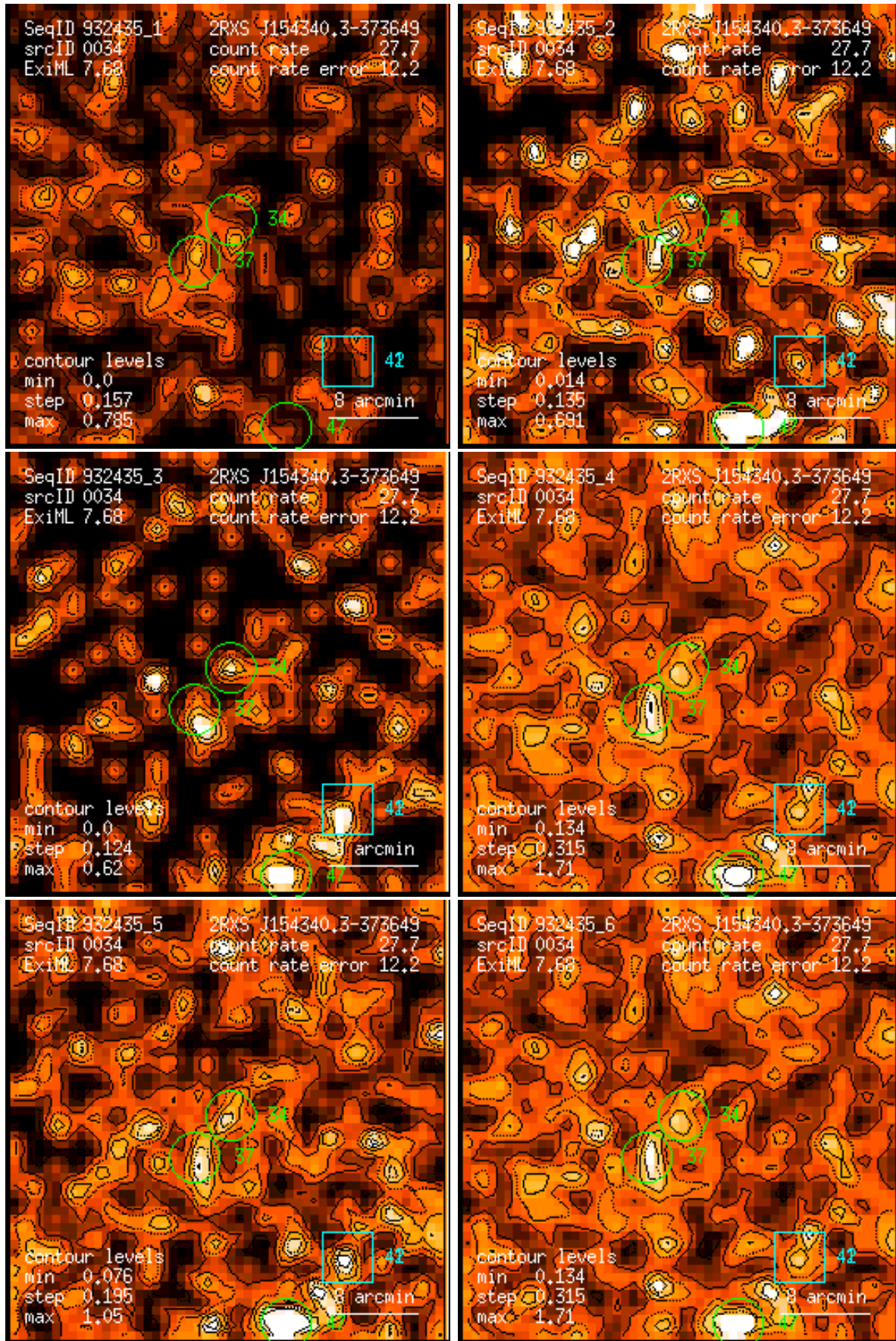
Figure 34: RASS 932435: detection 0034: band rate images, Gaussian filter: (1) PSPC channels 11 – 41, (2) 52 – 90, (3) 91 – 201, (4) 11 – 235, (5) 52 – 201, (6) 11 – 201. Broad band rates in counts/ks. Band rate contour levels in counts/ks/arcmin 2 .
