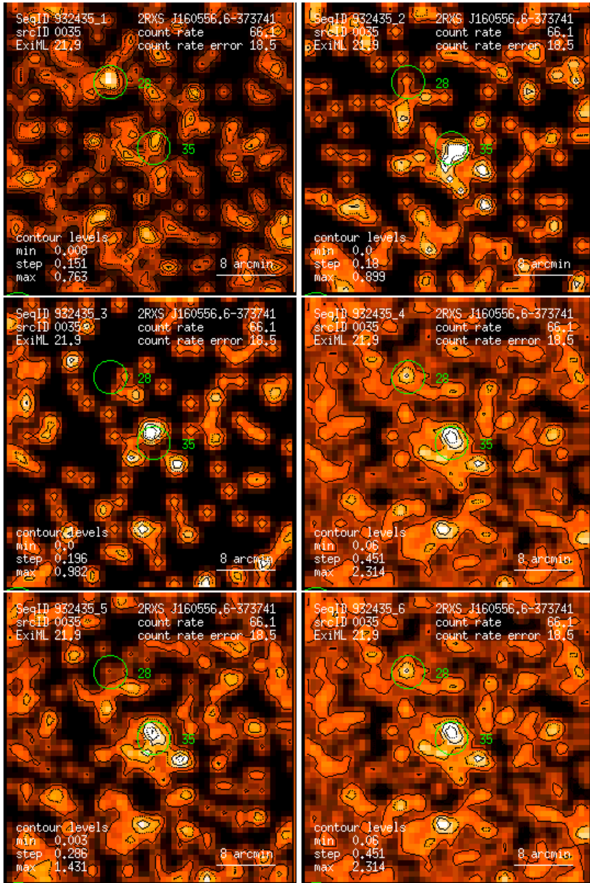
Figure 35: RASS 932435: detection 0035: band rate images, Gaussian filter: (1) PSPC channels 11 – 41, (2) 52 – 90, (3) 91 – 201, (4) 11 – 235, (5) 52 – 201, (6) 11 – 201. Broad band rates in counts/ks. Band rate contour levels in counts/ks/arcmin 2 .
