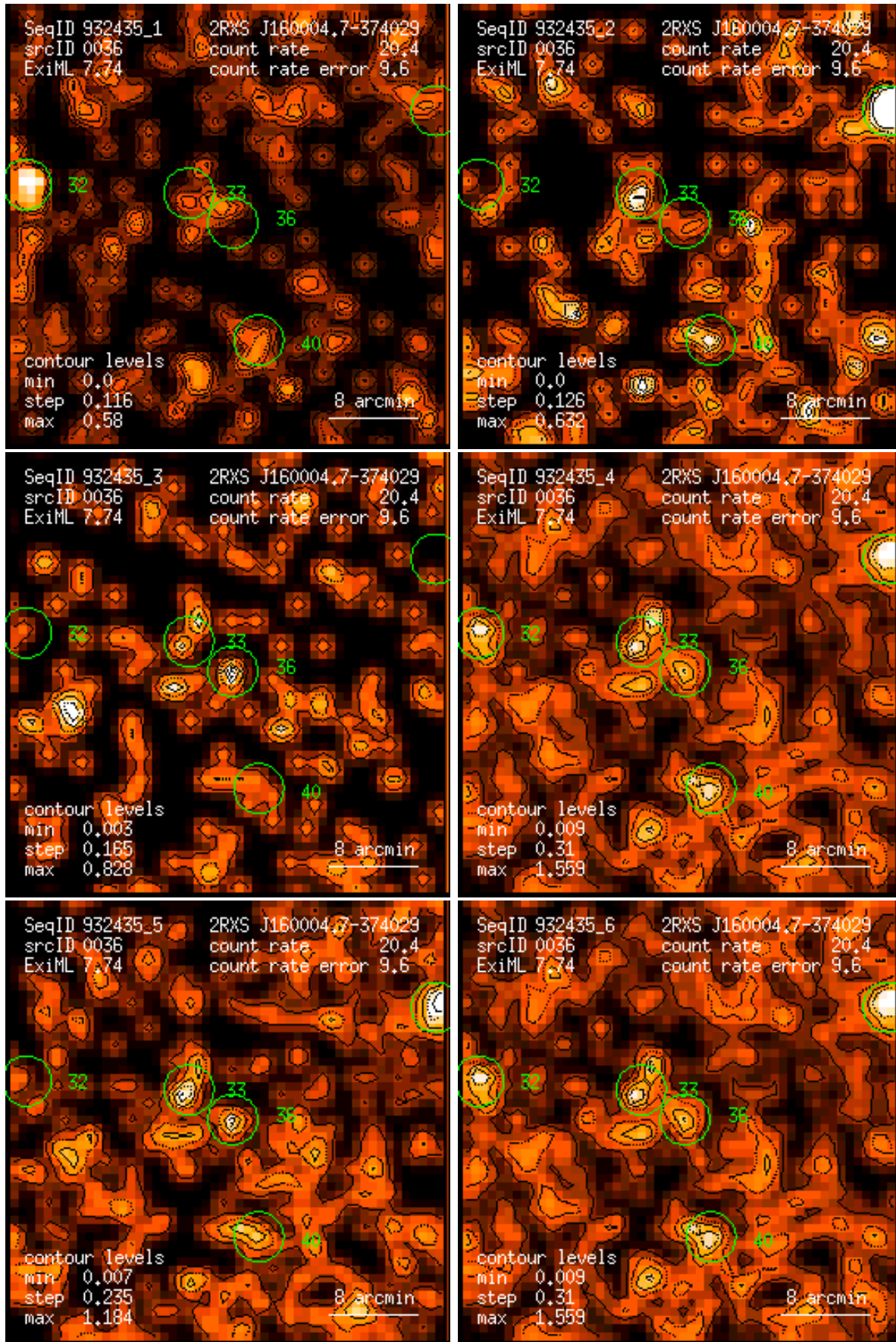
Figure 36: RASS 932435: detection 0036: band rate images, Gaussian filter: (1) PSPC channels 11 – 41, (2) 52 – 90, (3) 91 – 201, (4) 11 – 235, (5) 52 – 201, (6) 11 – 201. Broad band rates in counts/ks. Band rate contour levels in counts/ks/arcmin 2 .
