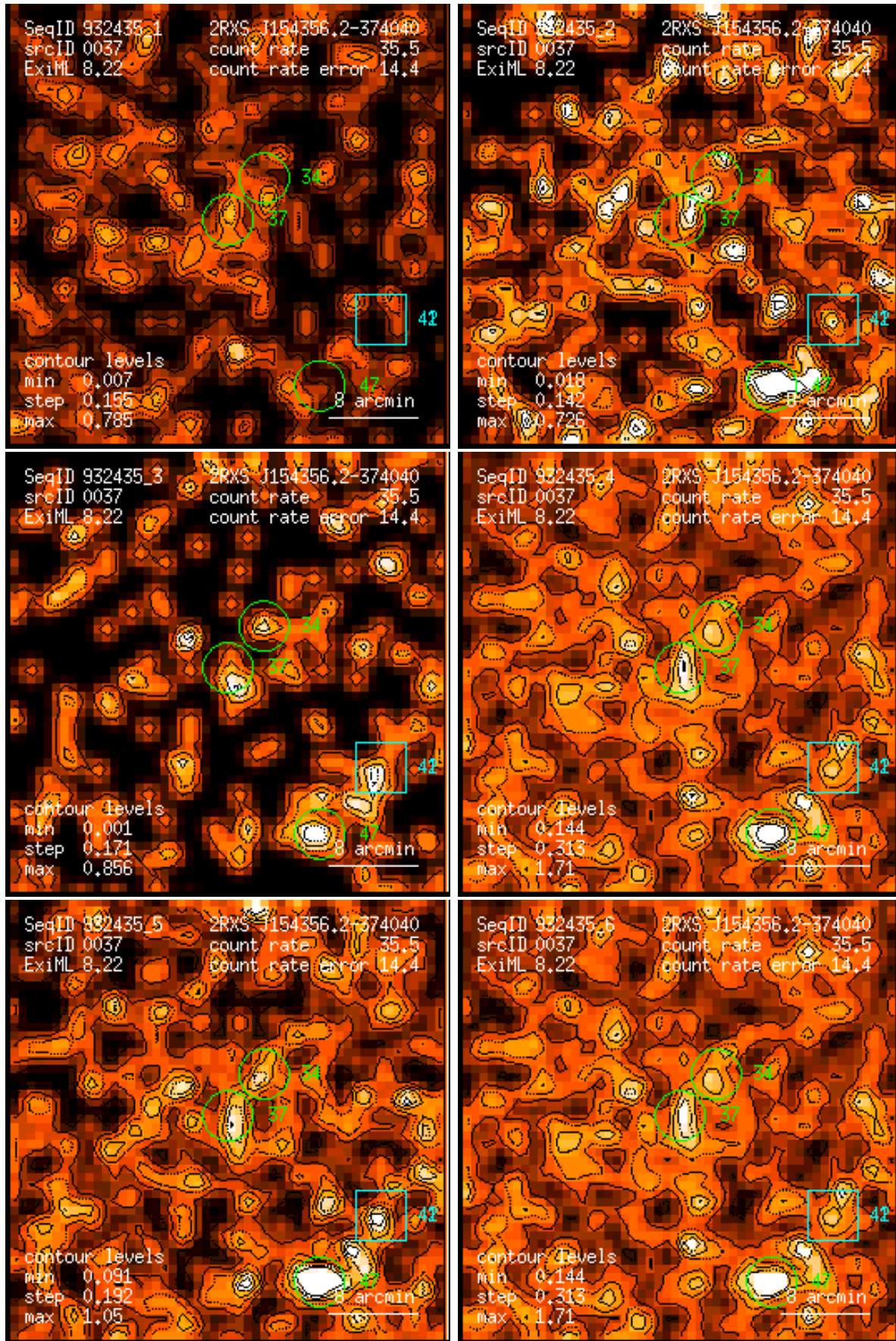
Figure 37: RASS 932435: detection 0037: band rate images, Gaussian filter: (1) PSPC channels 11 – 41, (2) 52 – 90, (3) 91 – 201, (4) 11 – 235, (5) 52 – 201, (6) 11 – 201. Broad band rates in counts/ks. Band rate contour levels in counts/ks/arcmin 2 .
