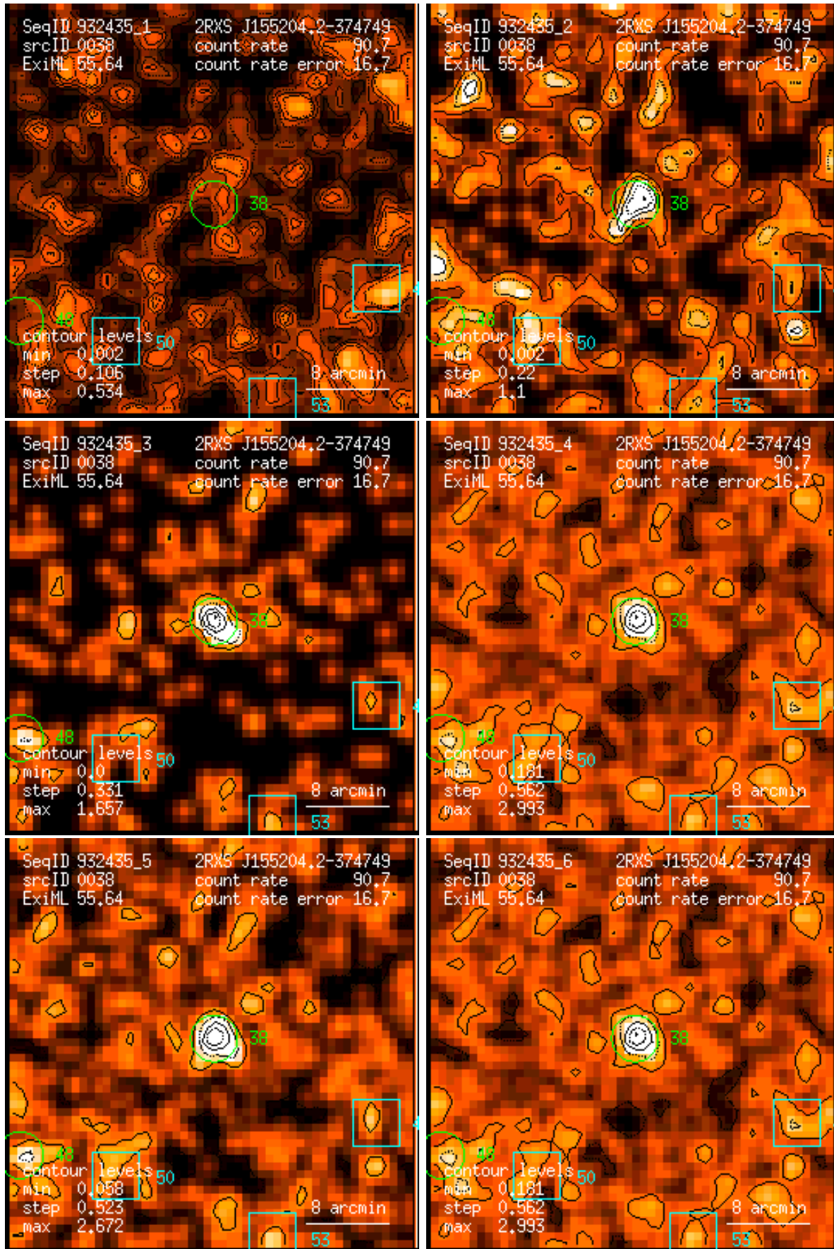
Figure 38: RASS 932435: detection 0038: band rate images, Gaussian filter: (1) PSPC channels 11 – 41, (2) 52 – 90, (3) 91 – 201, (4) 11 – 235, (5) 52 – 201, (6) 11 – 201. Broad band rates in counts/ks. Band rate contour levels in counts/ks/arcmin 2 .
