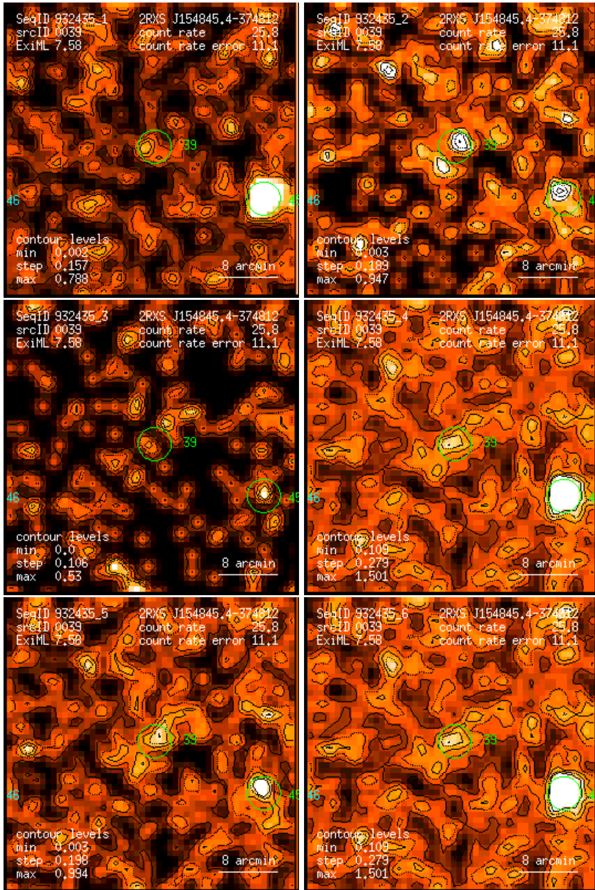
Figure 39: RASS 932435: detection 0039: band rate images, Gaussian filter: (1) PSPC channels 11 – 41, (2) 52 – 90, (3) 91 – 201, (4) 11 – 235, (5) 52 – 201, (6) 11 – 201. Broad band rates in counts/ks. Band rate contour levels in counts/ks/arcmin 2 .
