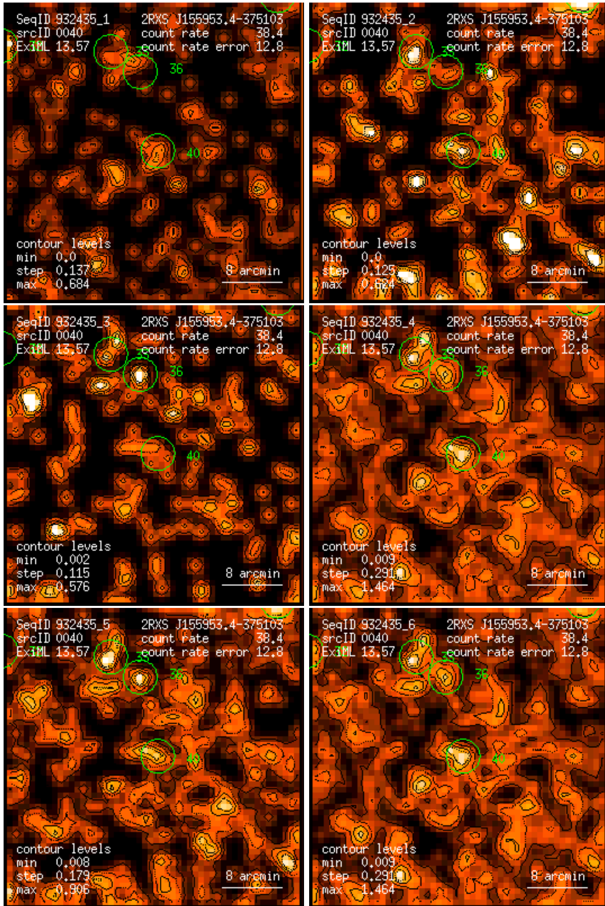
Figure 40: RASS 932435: detection 0040: band rate images, Gaussian filter: (1) PSPC channels 11 – 41, (2) 52 – 90, (3) 91 – 201, (4) 11 – 235, (5) 52 – 201, (6) 11 – 201. Broad band rates in counts/ks. Band rate contour levels in counts/ks/arcmin 2 .
