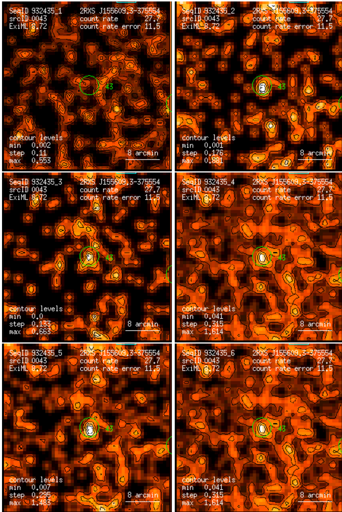
Figure 43: RASS 932435: detection 0043: band rate images, Gaussian filter: (1) PSPC channels 11 – 41, (2) 52 – 90, (3) 91 – 201, (4) 11 – 235, (5) 52 – 201, (6) 11 – 201. Broad band rates in counts/ks. Band rate contour levels in counts/ks/arcmin 2 .
