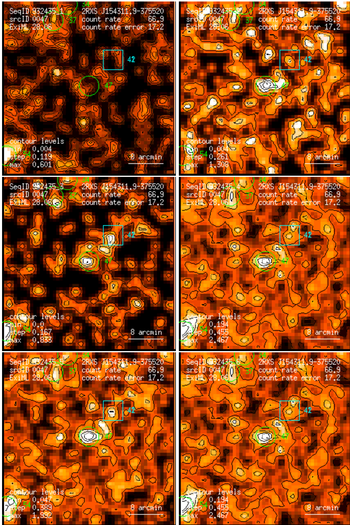
Figure 47: RASS 932435: detection 0047: band rate images, Gaussian filter: (1) PSPC channels 11 – 41, (2) 52 – 90, (3) 91 – 201, (4) 11 – 235, (5) 52 – 201, (6) 11 – 201. Broad band rates in counts/ks. Band rate contour levels in counts/ks/arcmin 2 .
