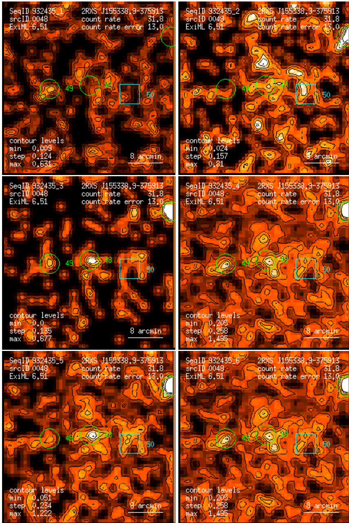
Figure 48: RASS 932435: detection 0048: band rate images, Gaussian filter: (1) PSPC channels 11 – 41, (2) 52 – 90, (3) 91 – 201, (4) 11 – 235, (5) 52 – 201, (6) 11 – 201. Broad band rates in counts/ks. Band rate contour levels in counts/ks/arcmin 2 .
