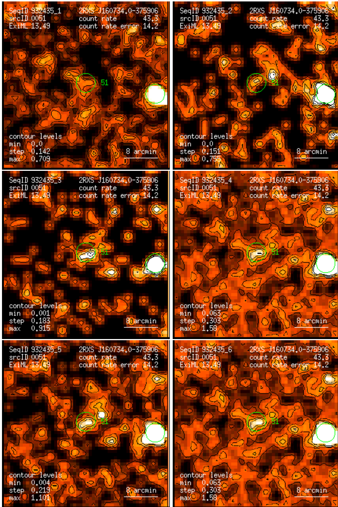
Figure 51: RASS 932435: detection 0051: band rate images, Gaussian filter: (1) PSPC channels 11 – 41, (2) 52 – 90, (3) 91 – 201, (4) 11 – 235, (5) 52 – 201, (6) 11 – 201. Broad band rates in counts/ks. Band rate contour levels in counts/ks/arcmin 2 .
