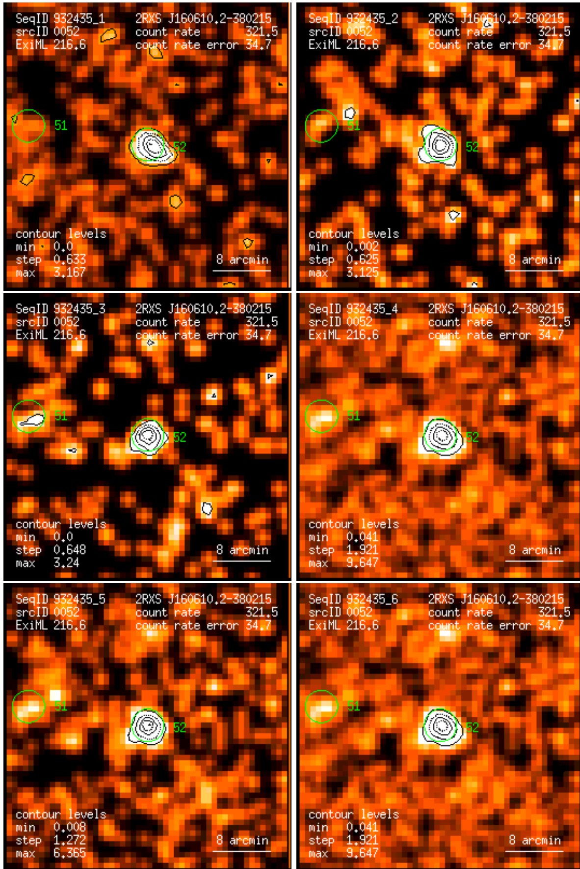
Figure 52: RASS 932435: detection 0052: band rate images, Gaussian filter: (1) PSPC channels 11 – 41, (2) 52 – 90, (3) 91 – 201, (4) 11 – 235, (5) 52 – 201, (6) 11 – 201. Broad band rates in counts/ks. Band rate contour levels in counts/ks/arcmin 2 .
