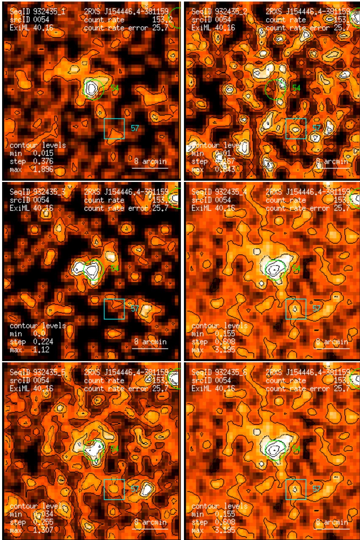
Figure 54: RASS 932435: detection 0054: band rate images, Gaussian filter: (1) PSPC channels 11 – 41, (2) 52 – 90, (3) 91 – 201, (4) 11 – 235, (5) 52 – 201, (6) 11 – 201. Broad band rates in counts/ks. Band rate contour levels in counts/ks/arcmin 2 .
