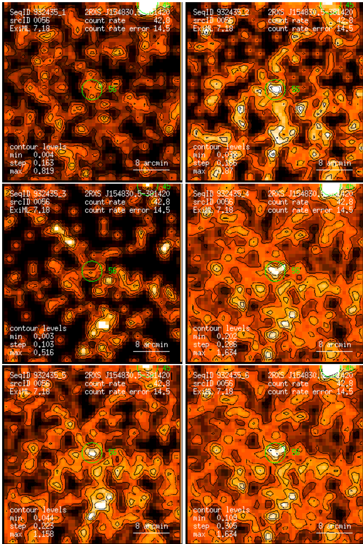
Figure 56: RASS 932435: detection 0056: band rate images, Gaussian filter: (1) PSPC channels 11 – 41, (2) 52 – 90, (3) 91 – 201, (4) 11 – 235, (5) 52 – 201, (6) 11 – 201. Broad band rates in counts/ks. Band rate contour levels in counts/ks/arcmin 2 .
