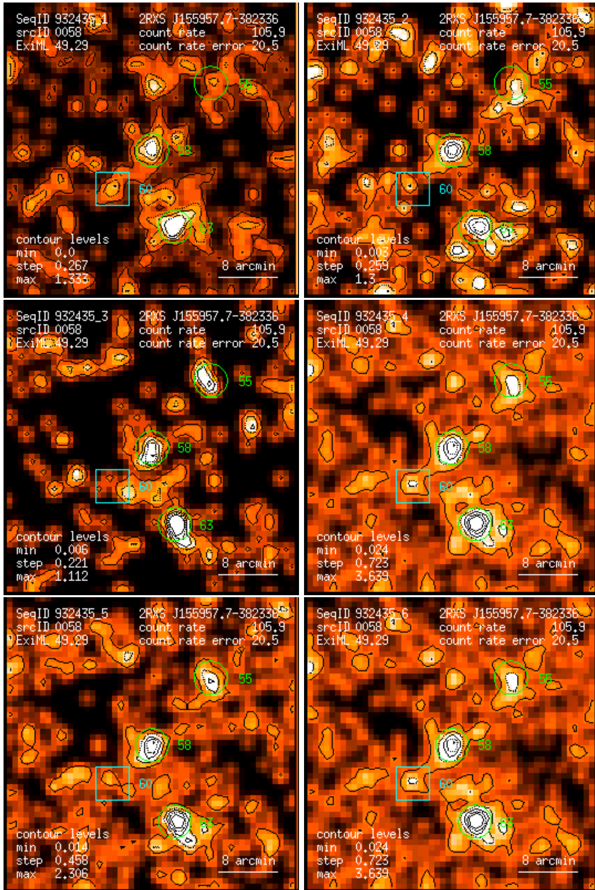
Figure 58: RASS 932435: detection 0058: band rate images, Gaussian filter: (1) PSPC channels 11 – 41, (2) 52 – 90, (3) 91 – 201, (4) 11 – 235, (5) 52 – 201, (6) 11 – 201. Broad band rates in counts/ks. Band rate contour levels in counts/ks/arcmin 2 .
