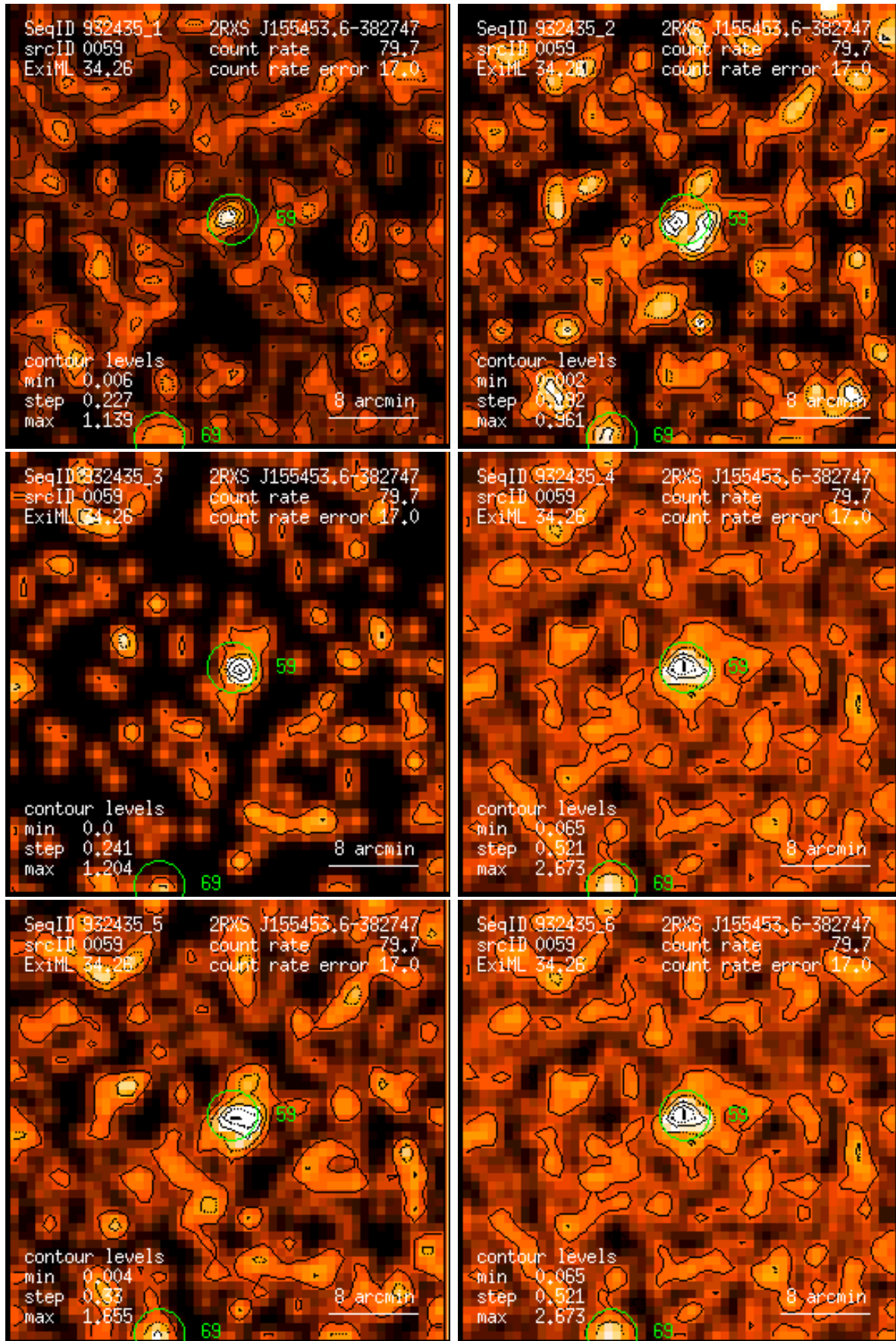
Figure 59: RASS 932435: detection 0059: band rate images, Gaussian filter: (1) PSPC channels 11 – 41, (2) 52 – 90, (3) 91 – 201, (4) 11 – 235, (5) 52 – 201, (6) 11 – 201. Broad band rates in counts/ks. Band rate contour levels in counts/ks/arcmin 2 .
