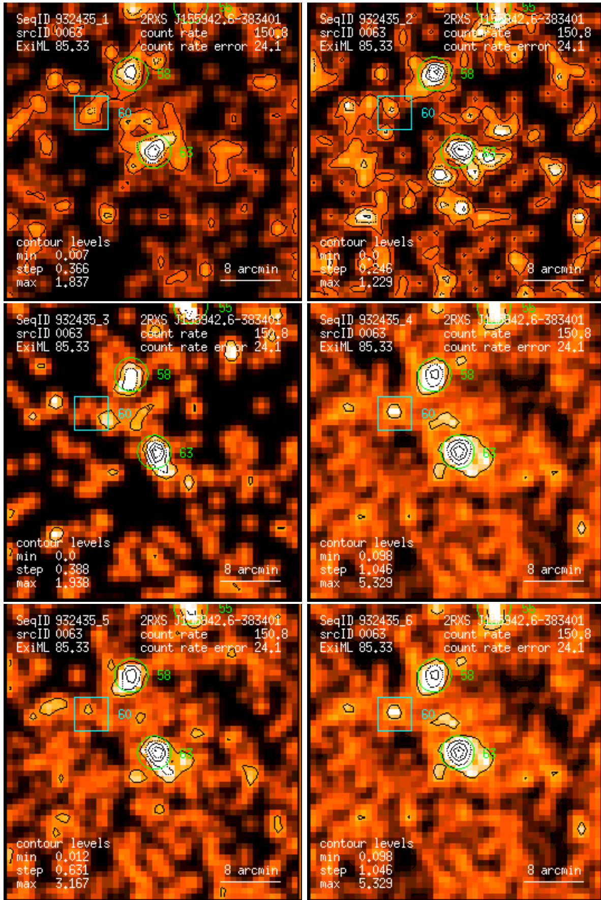
Figure 63: RASS 932435: detection 0063: band rate images, Gaussian filter: (1) PSPC channels 11 – 41, (2) 52 – 90, (3) 91 – 201, (4) 11 – 235, (5) 52 – 201, (6) 11 – 201. Broad band rates in counts/ks. Band rate contour levels in counts/ks/arcmin 2 .
