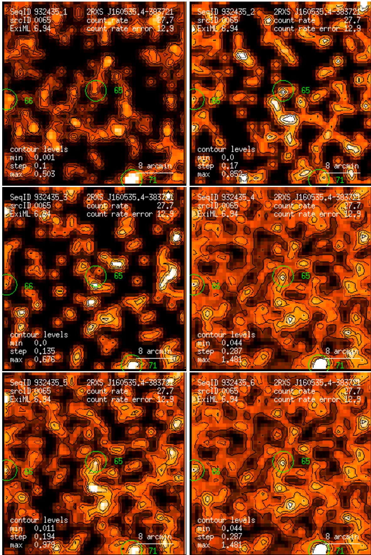
Figure 65: RASS 932435: detection 0065: band rate images, Gaussian filter: (1) PSPC channels 11 – 41, (2) 52 – 90, (3) 91 – 201, (4) 11 – 235, (5) 52 – 201, (6) 11 – 201. Broad band rates in counts/ks. Band rate contour levels in counts/ks/arcmin 2 .
