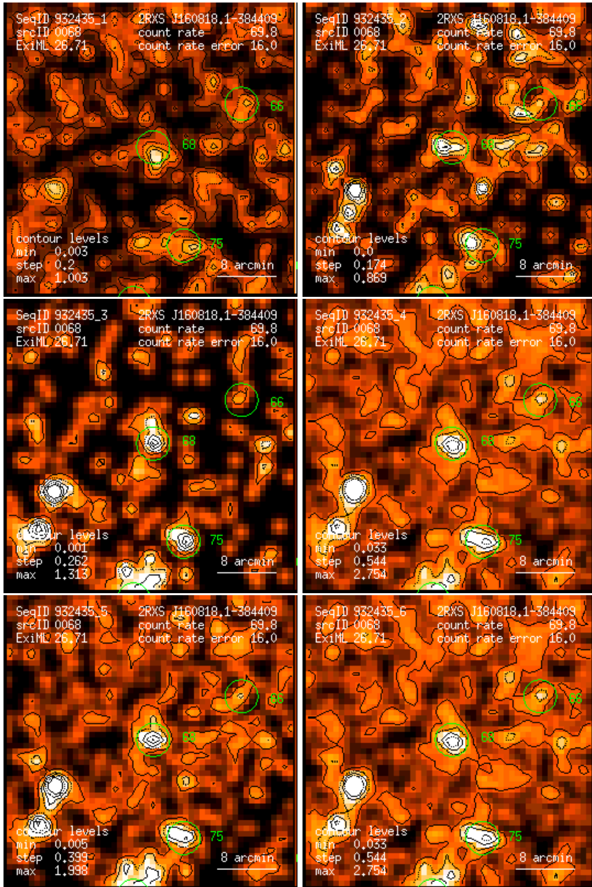
Figure 68: RASS 932435: detection 0068: band rate images, Gaussian filter: (1) PSPC channels 11 – 41, (2) 52 – 90, (3) 91 – 201, (4) 11 – 235, (5) 52 – 201, (6) 11 – 201. Broad band rates in counts/ks. Band rate contour levels in counts/ks/arcmin 2 .
