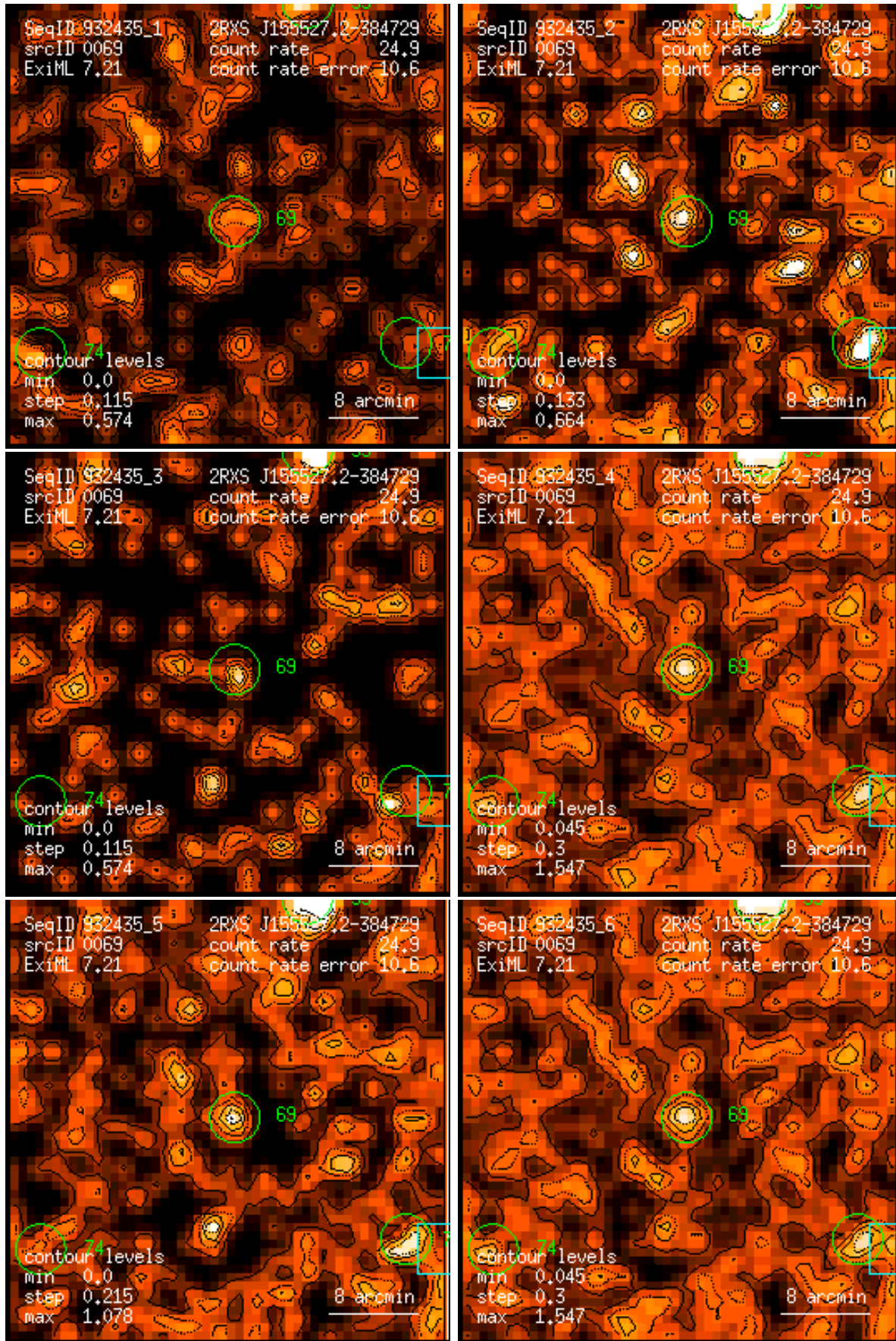
Figure 69: RASS 932435: detection 0069: band rate images, Gaussian filter: (1) PSPC channels 11 – 41, (2) 52 – 90, (3) 91 – 201, (4) 11 – 235, (5) 52 – 201, (6) 11 – 201. Broad band rates in counts/ks. Band rate contour levels in counts/ks/arcmin 2 .
