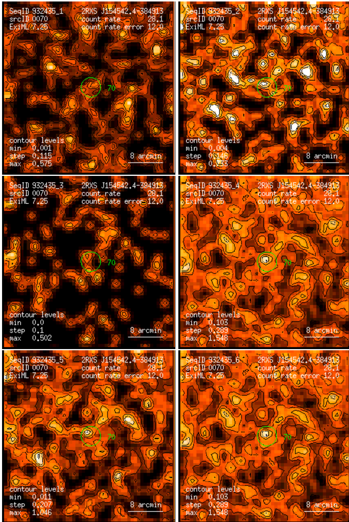
Figure 70: RASS 932435: detection 0070: band rate images, Gaussian filter: (1) PSPC channels 11 – 41, (2) 52 – 90, (3) 91 – 201, (4) 11 – 235, (5) 52 – 201, (6) 11 – 201. Broad band rates in counts/ks. Band rate contour levels in counts/ks/arcmin 2 .
