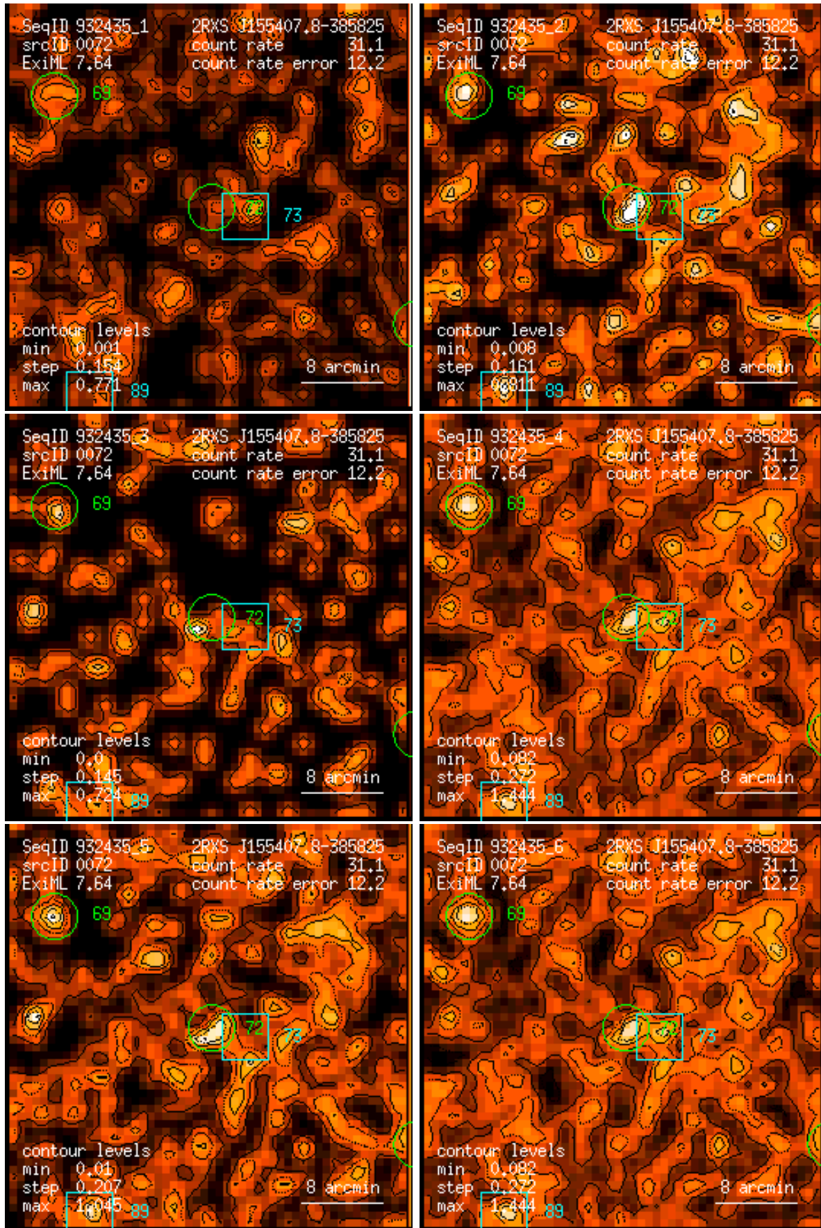
Figure 72: RASS 932435: detection 0072: band rate images, Gaussian filter: (1) PSPC channels 11 – 41, (2) 52 – 90, (3) 91 – 201, (4) 11 – 235, (5) 52 – 201, (6) 11 – 201. Broad band rates in counts/ks. Band rate contour levels in counts/ks/arcmin 2 .
