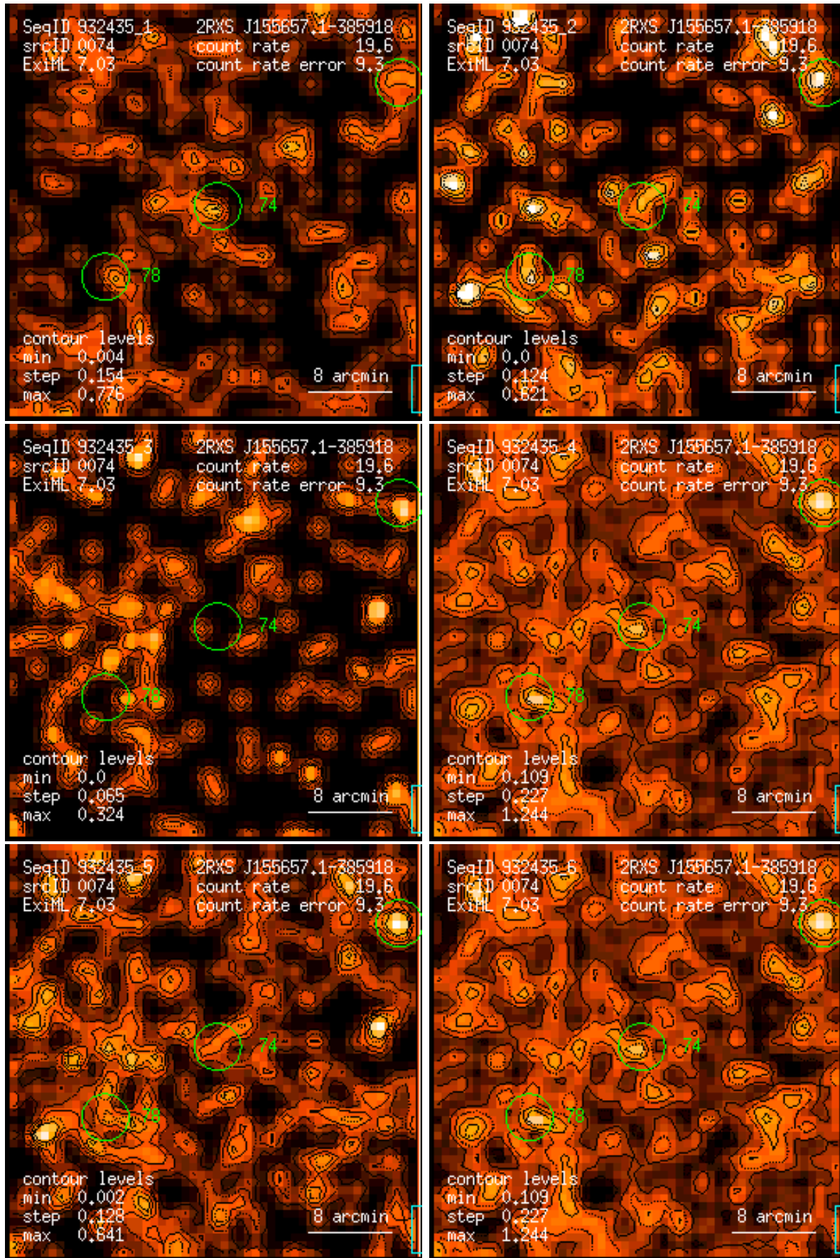
Figure 74: RASS 932435: detection 0074: band rate images, Gaussian filter: (1) PSPC channels 11 – 41, (2) 52 – 90, (3) 91 – 201, (4) 11 – 235, (5) 52 – 201, (6) 11 – 201. Broad band rates in counts/ks. Band rate contour levels in counts/ks/arcmin 2 .
