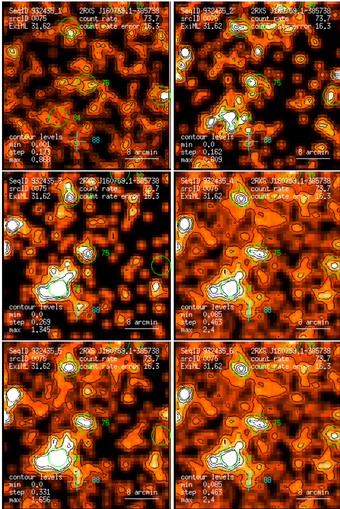
Figure 75: RASS 932435: detection 0075: band rate images, Gaussian filter: (1) PSPC channels 11 – 41, (2) 52 – 90, (3) 91 – 201, (4) 11 – 235, (5) 52 – 201, (6) 11 – 201. Broad band rates in counts/ks. Band rate contour levels in counts/ks/arcmin 2 .
