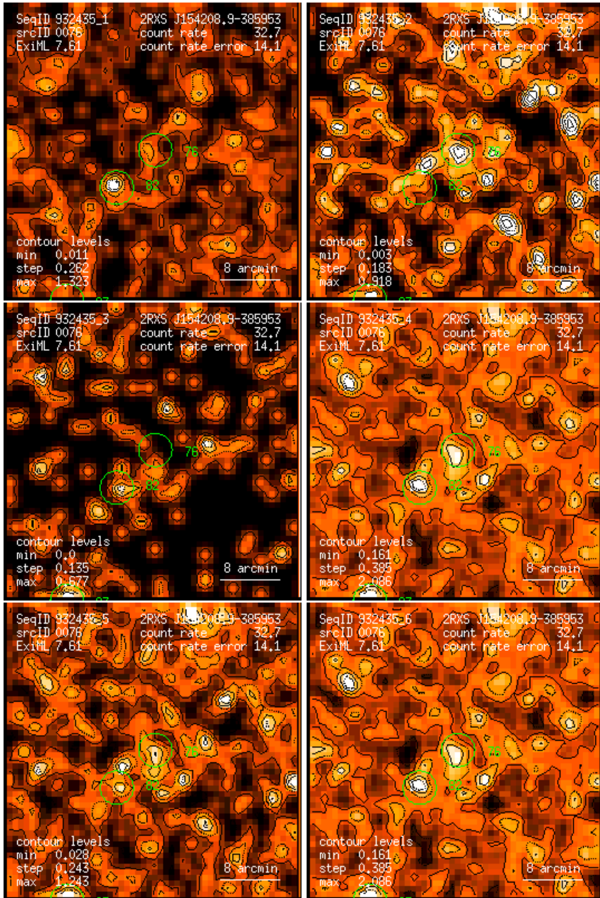
Figure 76: RASS 932435: detection 0076: band rate images, Gaussian filter: (1) PSPC channels 11 – 41, (2) 52 – 90, (3) 91 – 201, (4) 11 – 235, (5) 52 – 201, (6) 11 – 201. Broad band rates in counts/ks. Band rate contour levels in counts/ks/arcmin 2 .
