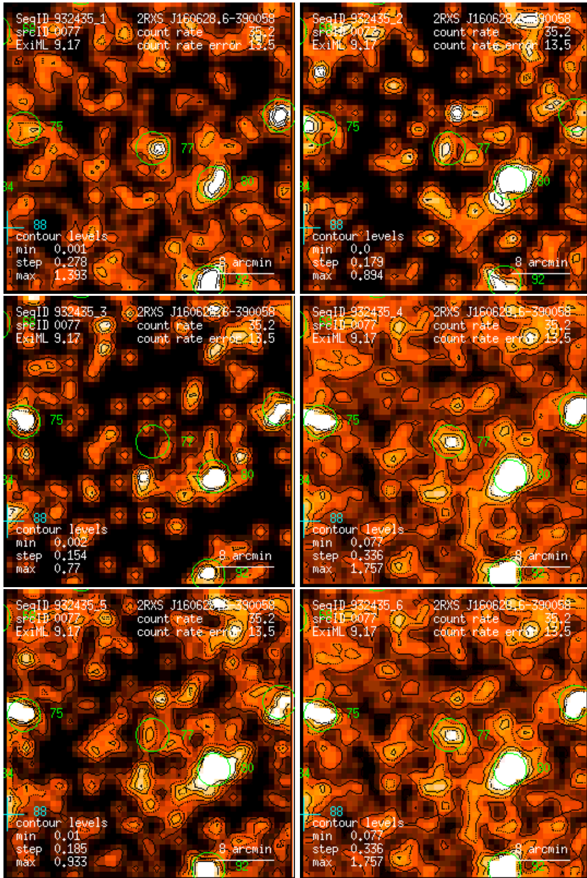
Figure 77: RASS 932435: detection 0077: band rate images, Gaussian filter: (1) PSPC channels 11 – 41, (2) 52 – 90, (3) 91 – 201, (4) 11 – 235, (5) 52 – 201, (6) 11 – 201. Broad band rates in counts/ks. Band rate contour levels in counts/ks/arcmin 2 .
