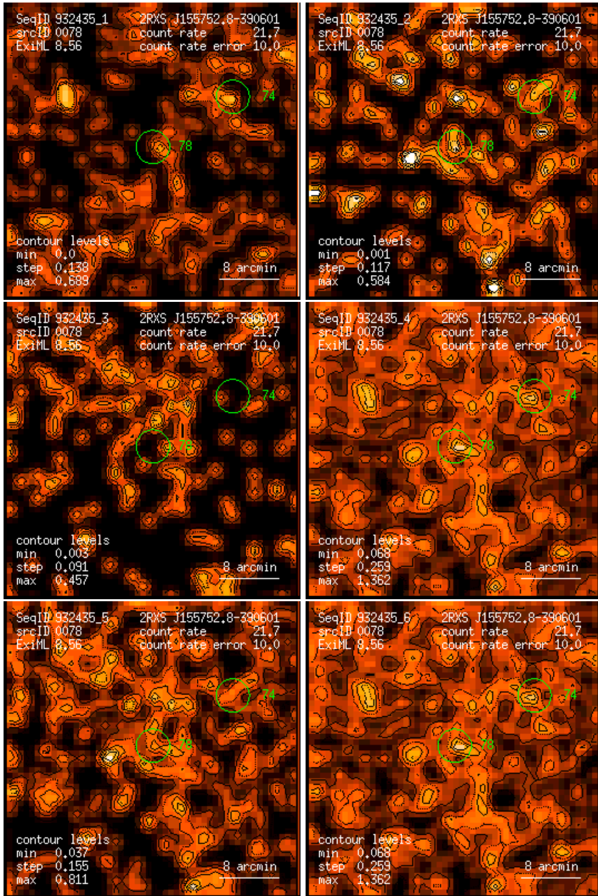
Figure 78: RASS 932435: detection 0078: band rate images, Gaussian filter: (1) PSPC channels 11 – 41, (2) 52 – 90, (3) 91 – 201, (4) 11 – 235, (5) 52 – 201, (6) 11 – 201. Broad band rates in counts/ks. Band rate contour levels in counts/ks/arcmin 2 .
