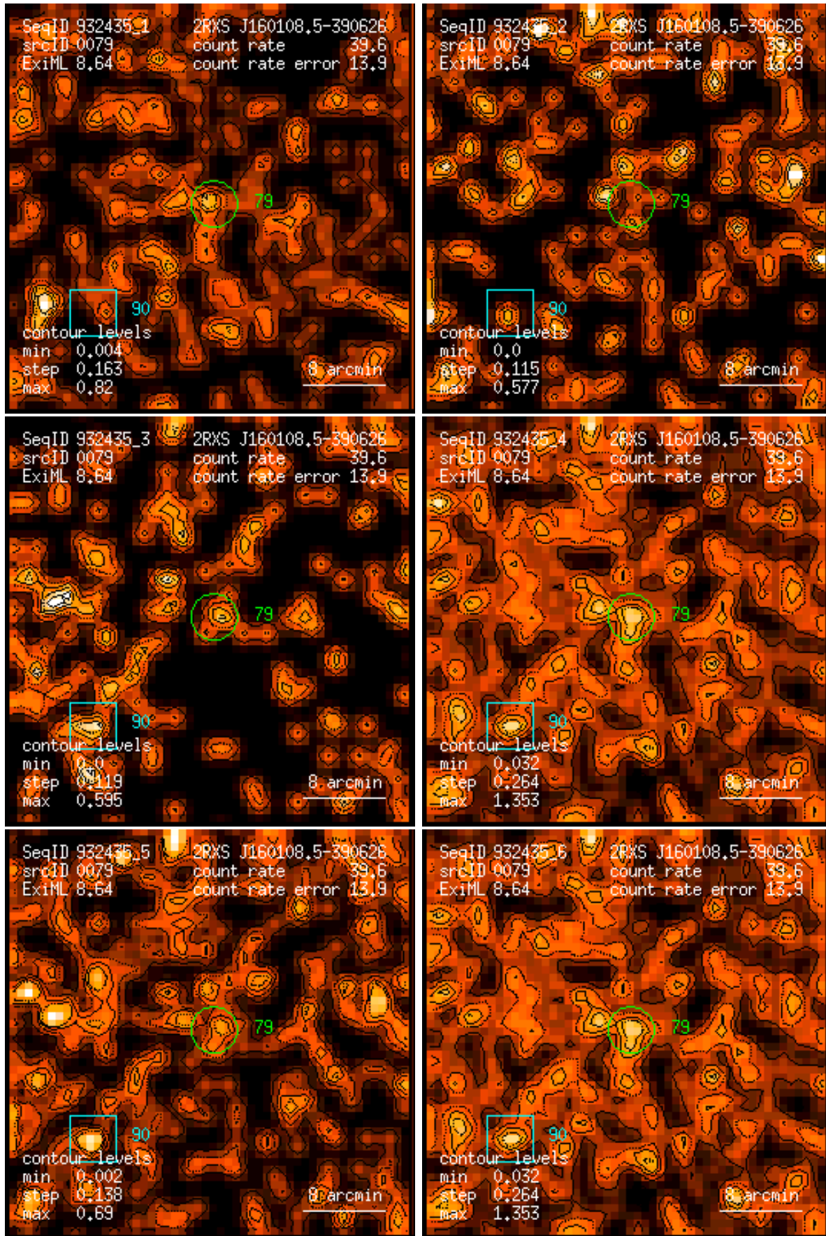
Figure 79: RASS 932435: detection 0079: band rate images, Gaussian filter: (1) PSPC channels 11 – 41, (2) 52 – 90, (3) 91 – 201, (4) 11 – 235, (5) 52 – 201, (6) 11 – 201. Broad band rates in counts/ks. Band rate contour levels in counts/ks/arcmin 2 .
