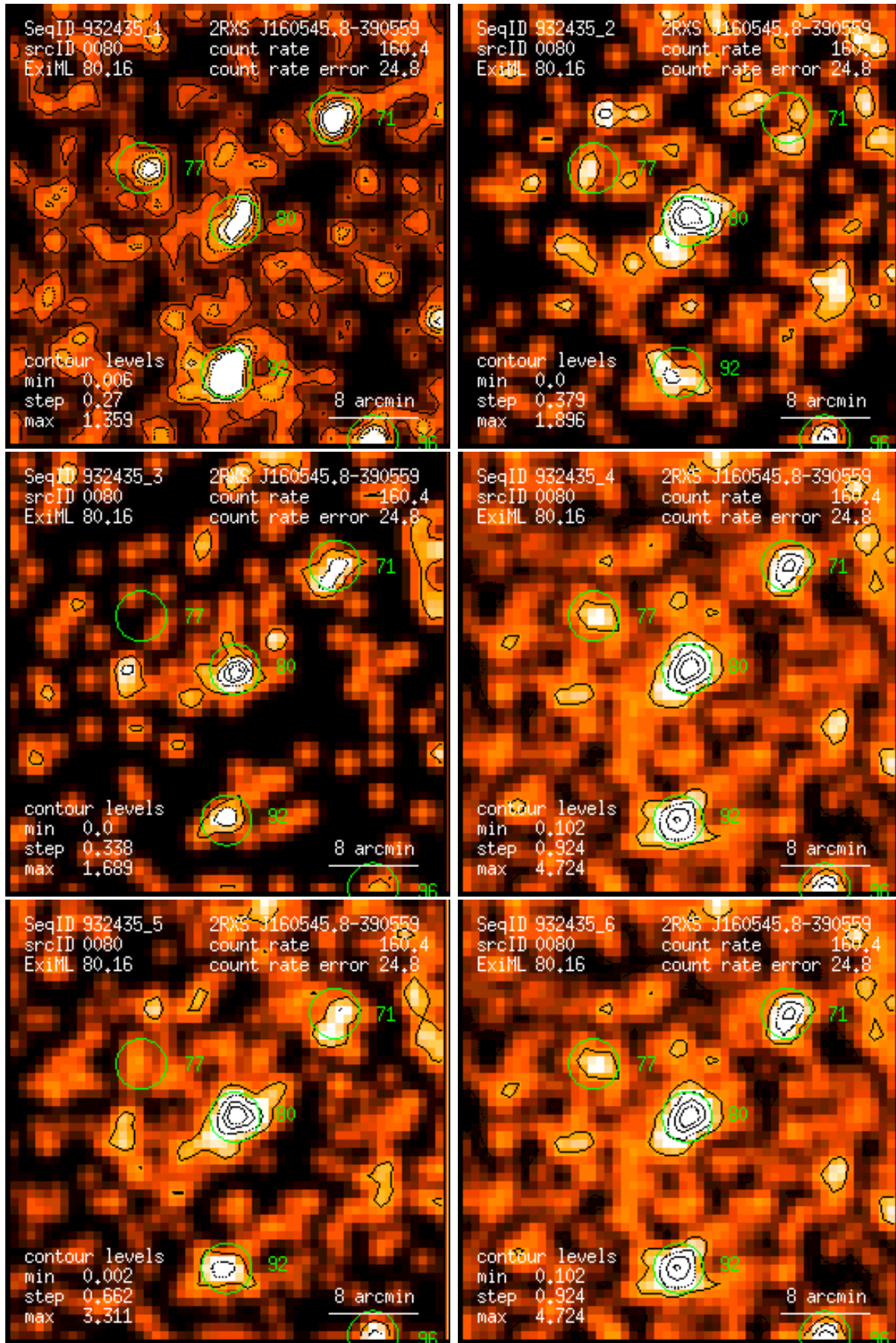
Figure 80: RASS 932435: detection 0080: band rate images, Gaussian filter: (1) PSPC channels 11 – 41, (2) 52 – 90, (3) 91 – 201, (4) 11 – 235, (5) 52 – 201, (6) 11 – 201. Broad band rates in counts/ks. Band rate contour levels in counts/ks/arcmin 2 .
