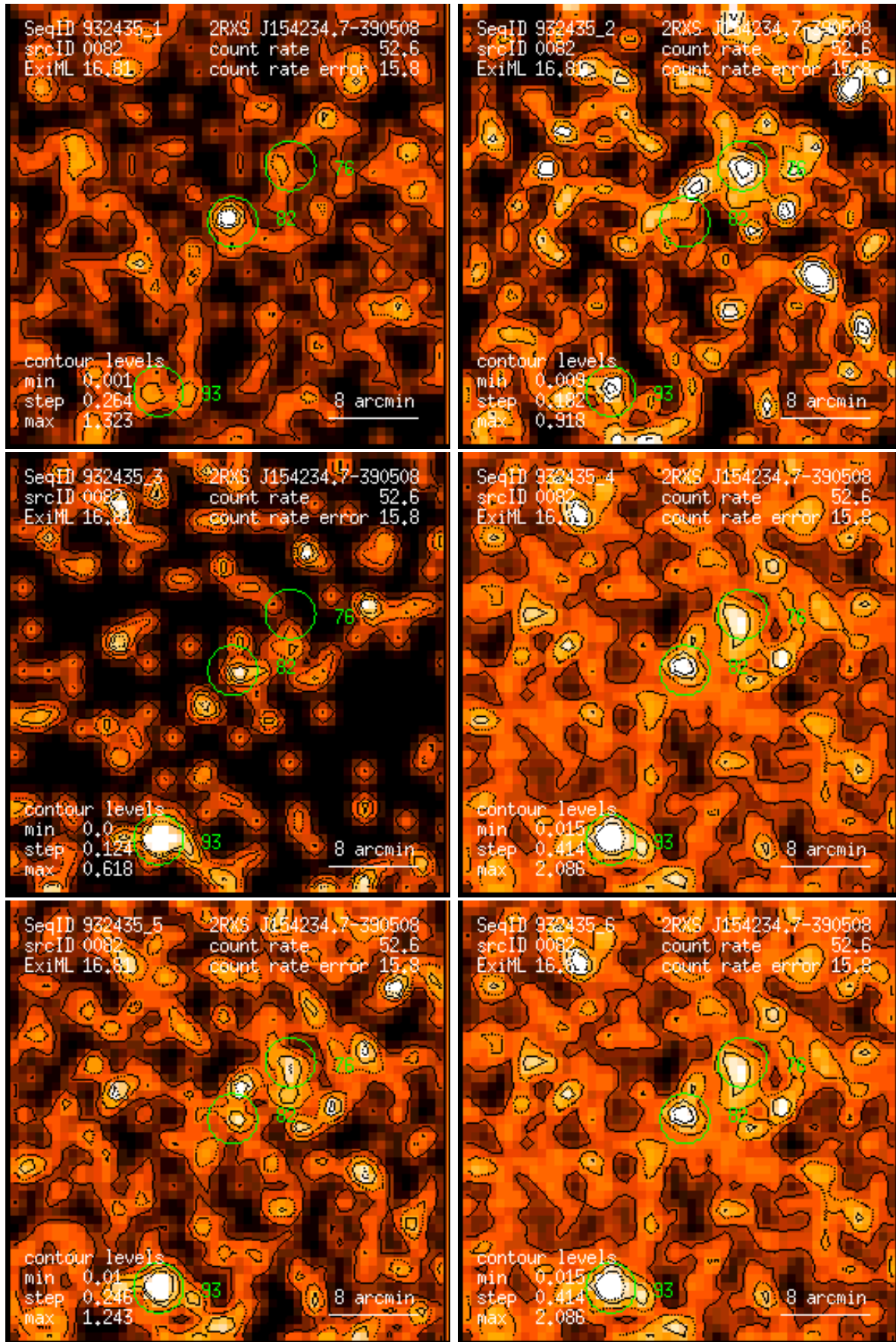
Figure 82: RASS 932435: detection 0082: band rate images, Gaussian filter: (1) PSPC channels 11 – 41, (2) 52 – 90, (3) 91 – 201, (4) 11 – 235, (5) 52 – 201, (6) 11 – 201. Broad band rates in counts/ks. Band rate contour levels in counts/ks/arcmin 2 .
