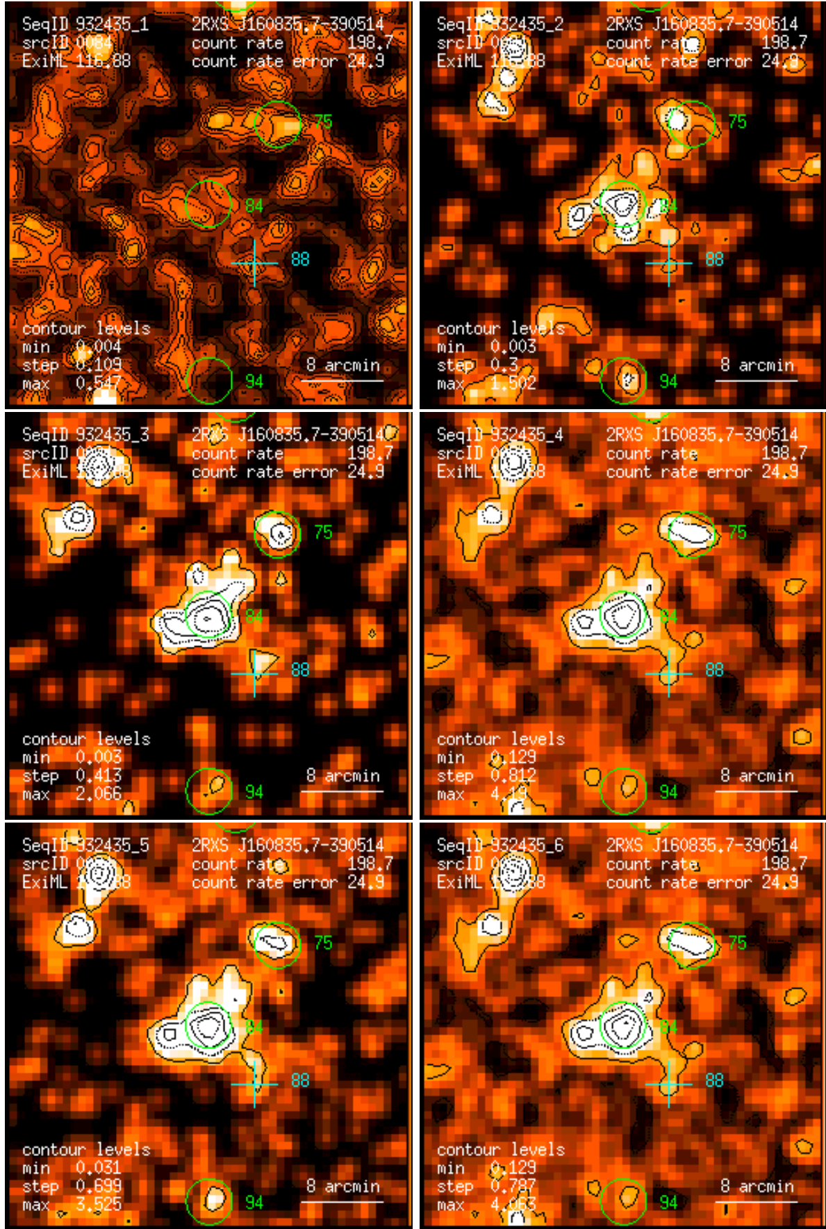
Figure 84: RASS 932435: detection 0084: band rate images, Gaussian filter: (1) PSPC channels 11 – 41, (2) 52 – 90, (3) 91 – 201, (4) 11 – 235, (5) 52 – 201, (6) 11 – 201. Broad band rates in counts/ks. Band rate contour levels in counts/ks/arcmin 2 .
