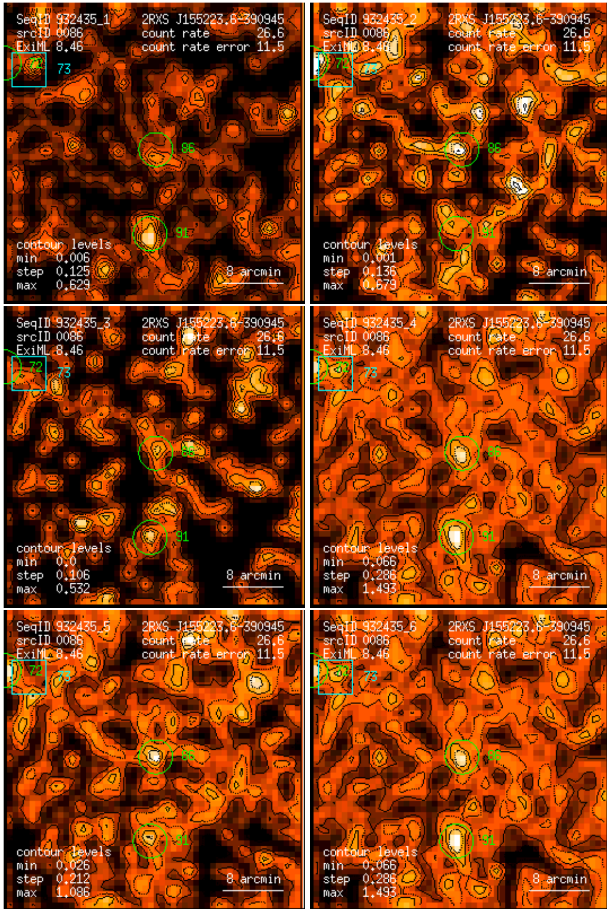
Figure 86: RASS 932435: detection 0086: band rate images, Gaussian filter: (1) PSPC channels 11 – 41, (2) 52 – 90, (3) 91 – 201, (4) 11 – 235, (5) 52 – 201, (6) 11 – 201. Broad band rates in counts/ks. Band rate contour levels in counts/ks/arcmin 2 .
