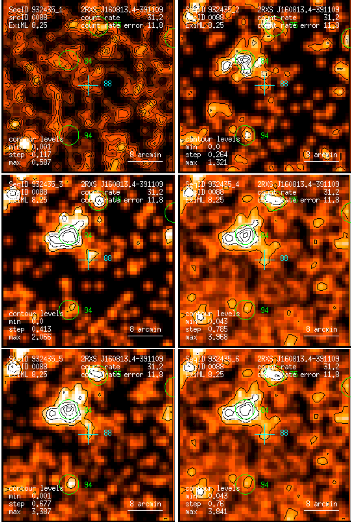
Figure 88: RASS 932435: detection 0088: band rate images, Gaussian filter: (1) PSPC channels 11 – 41, (2) 52 – 90, (3) 91 – 201, (4) 11 – 235, (5) 52 – 201, (6) 11 – 201. Broad band rates in counts/ks. Band rate contour levels in counts/ks/arcmin 2 .
