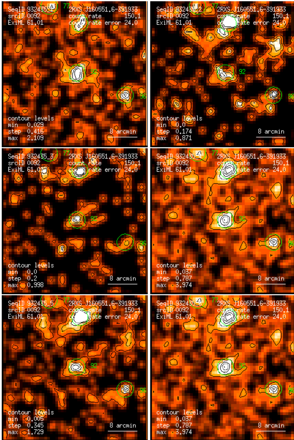
Figure 92: RASS 932435: detection 0092: band rate images, Gaussian filter: (1) PSPC channels 11 – 41, (2) 52 – 90, (3) 91 – 201, (4) 11 – 235, (5) 52 – 201, (6) 11 – 201. Broad band rates in counts/ks. Band rate contour levels in counts/ks/arcmin 2 .
